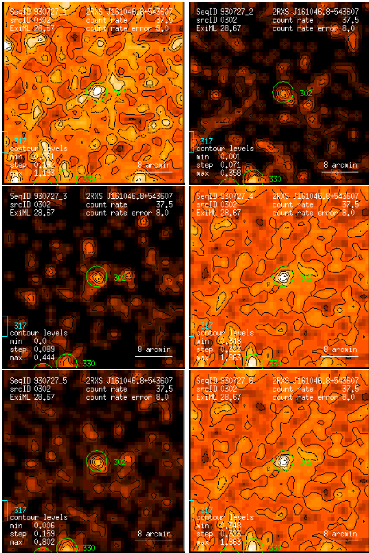
Figure 302: RASS 930727: detection 0302: band rate images, Gaussian filter: (1) PSPC channels 11 – 41, (2) 52 – 90, (3) 91 – 201, (4) 11 – 235, (5) 52 – 201, (6) 11 – 201. Broad band rates in counts/ks. Band rate contour levels in counts/ks/arcmin 2 .
