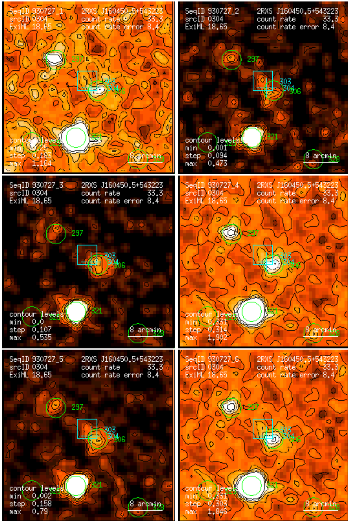
Figure 304: RASS 930727: detection 0304: band rate images, Gaussian filter: (1) PSPC channels 11 – 41, (2) 52 – 90, (3) 91 – 201, (4) 11 – 235, (5) 52 – 201, (6) 11 – 201. Broad band rates in counts/ks. Band rate contour levels in counts/ks/arcmin 2 .
