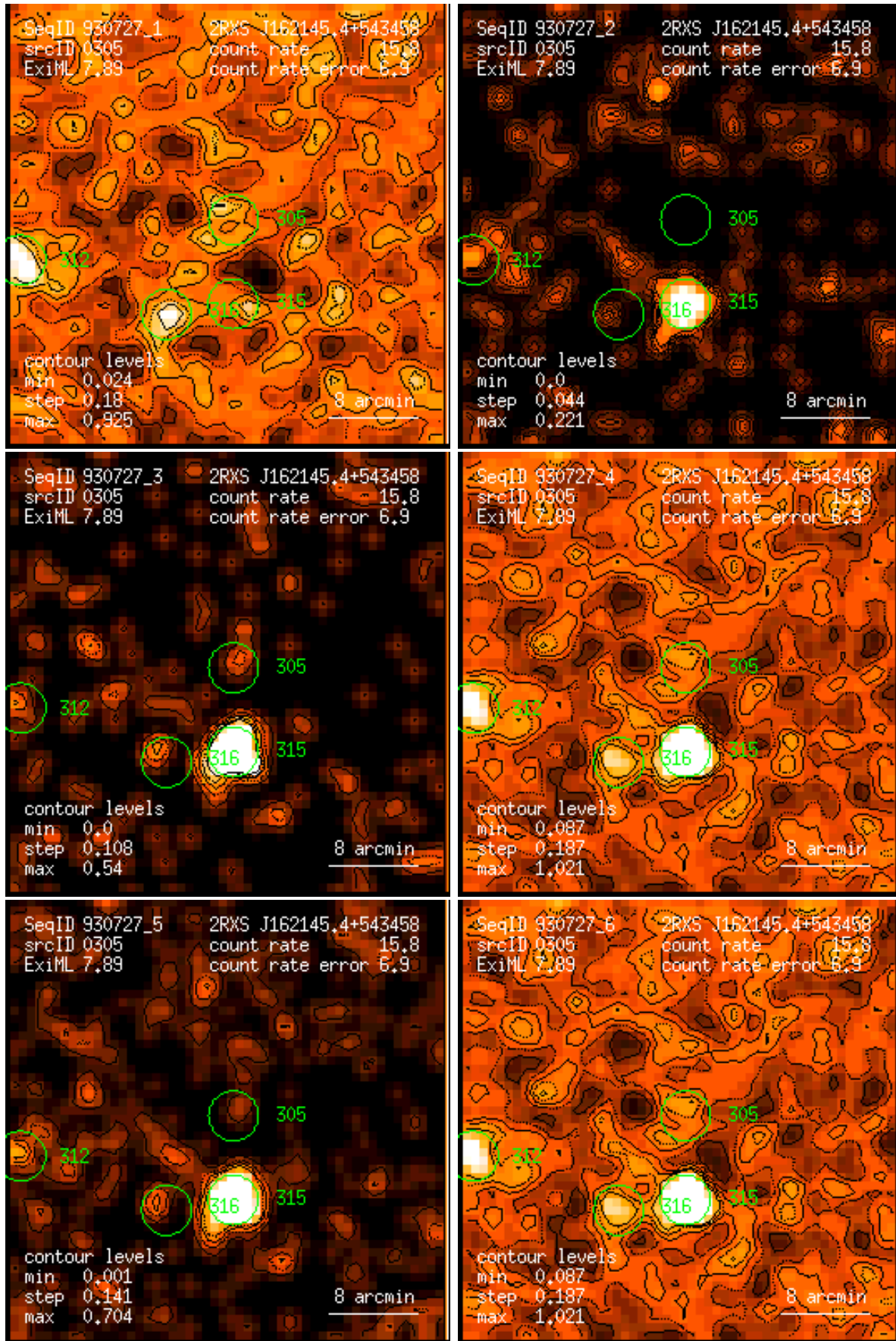
Figure 305: RASS 930727: detection 0305: band rate images, Gaussian filter: (1) PSPC channels 11 – 41, (2) 52 – 90, (3) 91 – 201, (4) 11 – 235, (5) 52 – 201, (6) 11 – 201. Broad band rates in counts/ks. Band rate contour levels in counts/ks/arcmin 2 .
