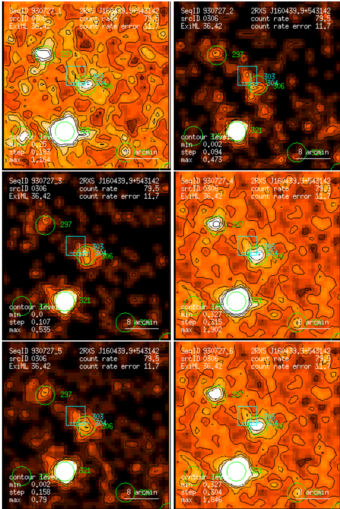
Figure 306: RASS 930727: detection 0306: band rate images, Gaussian filter: (1) PSPC channels 11 – 41, (2) 52 – 90, (3) 91 – 201, (4) 11 – 235, (5) 52 – 201, (6) 11 – 201. Broad band rates in counts/ks. Band rate contour levels in counts/ks/arcmin 2 .
