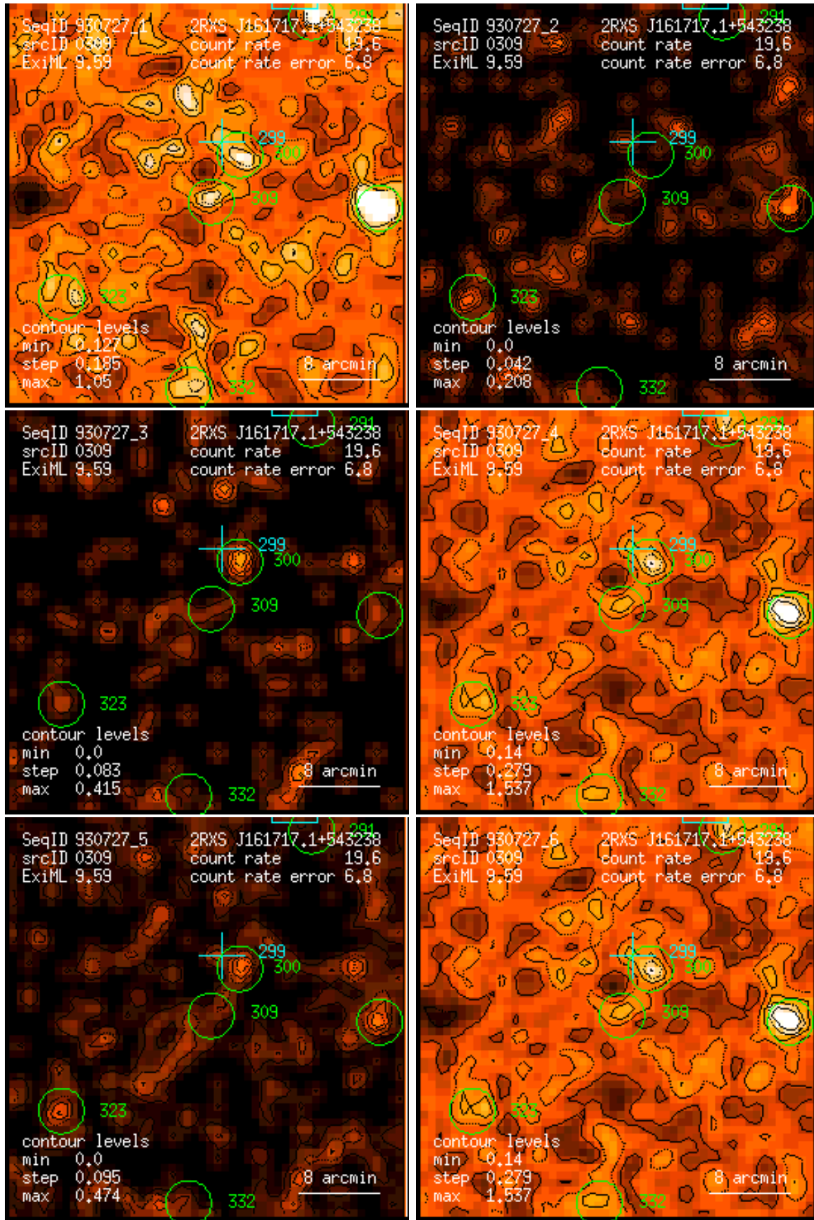
Figure 309: RASS 930727: detection 0309: band rate images, Gaussian filter: (1) PSPC channels 11 – 41, (2) 52 – 90, (3) 91 – 201, (4) 11 – 235, (5) 52 – 201, (6) 11 – 201. Broad band rates in counts/ks. Band rate contour levels in counts/ks/arcmin 2 .
