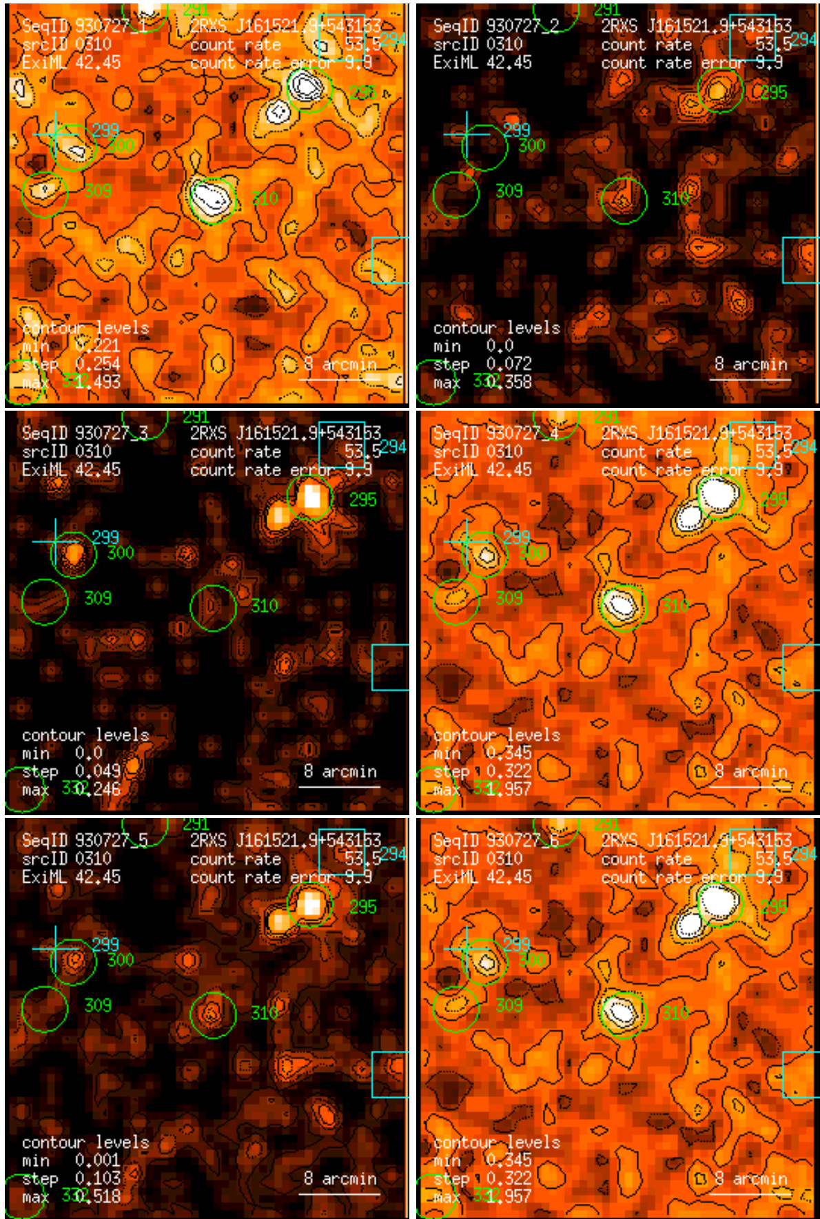
Figure 310: RASS 930727: detection 0310: band rate images, Gaussian filter: (1) PSPC channels 11 – 41, (2) 52 – 90, (3) 91 – 201, (4) 11 – 235, (5) 52 – 201, (6) 11 – 201. Broad band rates in counts/ks. Band rate contour levels in counts/ks/arcmin 2 .
