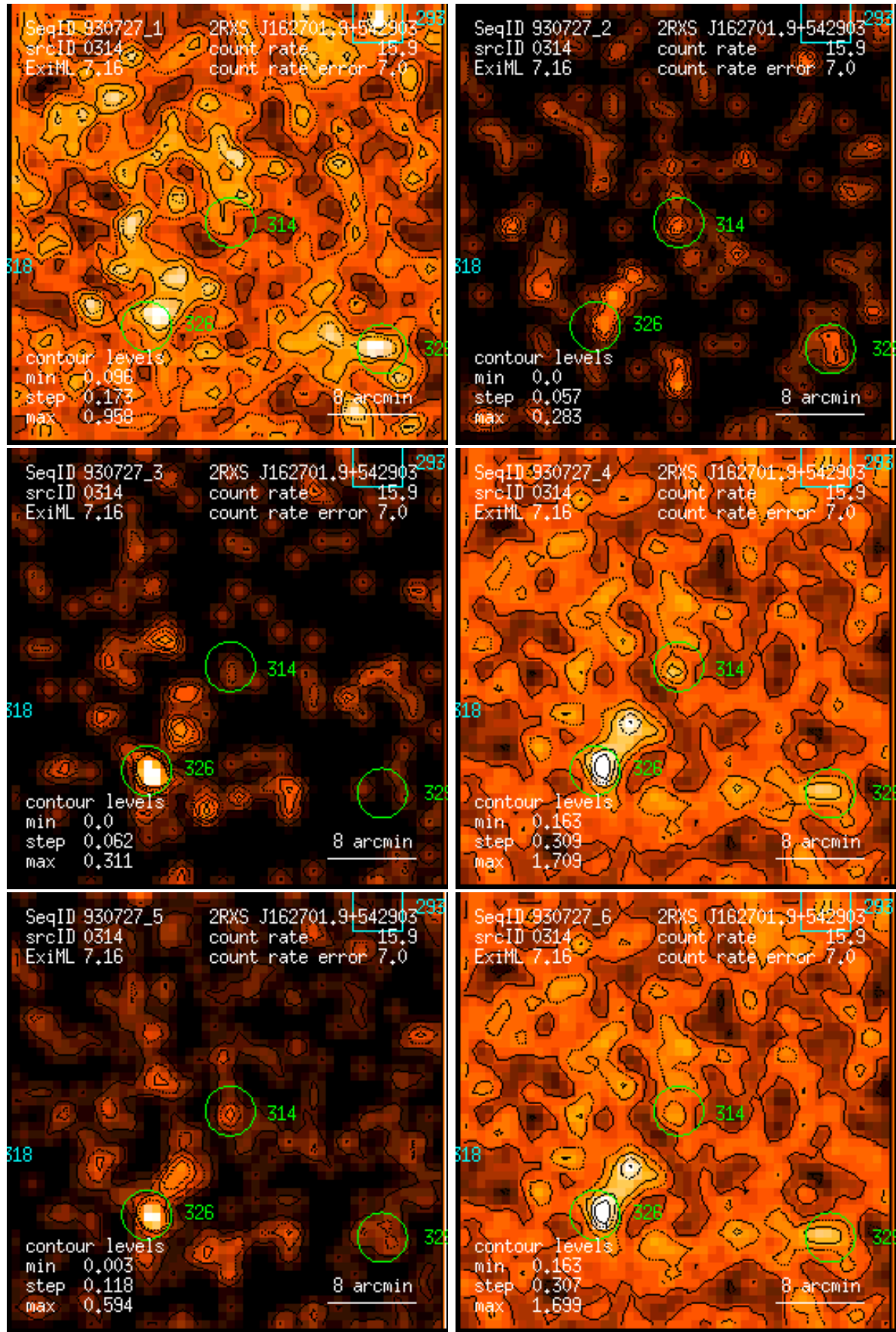
Figure 314: RASS 930727: detection 0314: band rate images, Gaussian filter: (1) PSPC channels 11 – 41, (2) 52 – 90, (3) 91 – 201, (4) 11 – 235, (5) 52 – 201, (6) 11 – 201. Broad band rates in counts/ks. Band rate contour levels in counts/ks/arcmin 2 .
