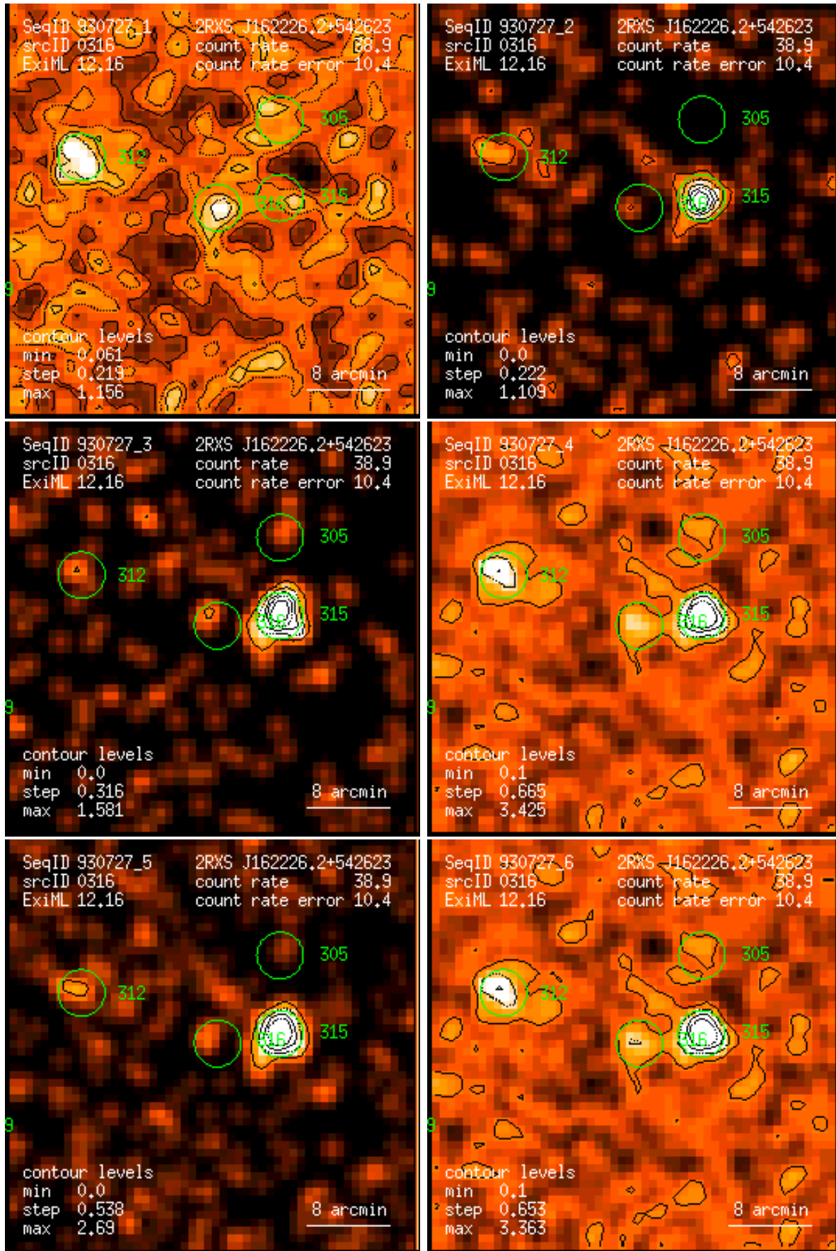
Figure 316: RASS 930727: detection 0316: band rate images, Gaussian filter: (1) PSPC channels 11 – 41, (2) 52 – 90, (3) 91 – 201, (4) 11 – 235, (5) 52 – 201, (6) 11 – 201. Broad band rates in counts/ks. Band rate contour levels in counts/ks/arcmin 2 .
