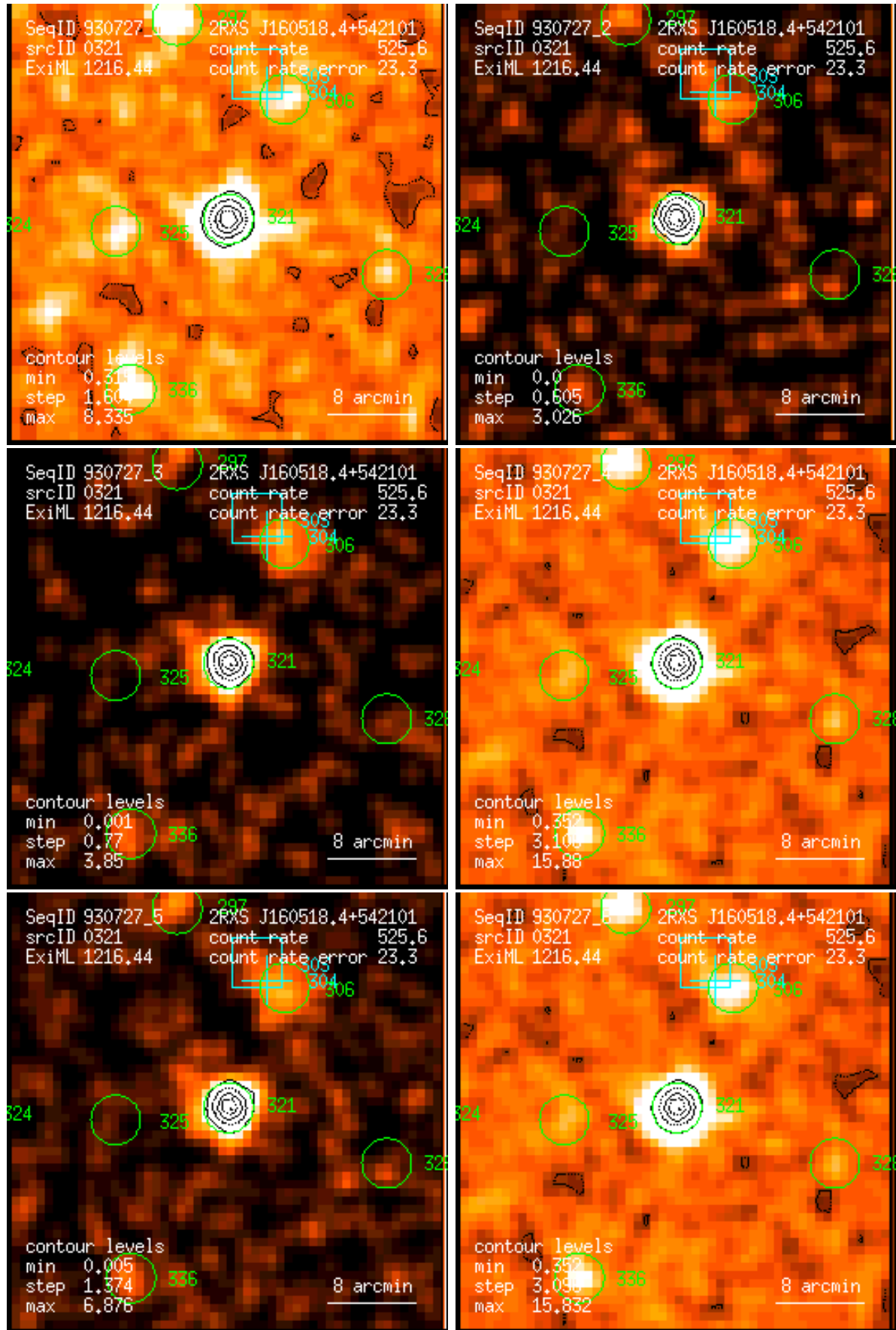
Figure 321: RASS 930727: detection 0321: band rate images, Gaussian filter: (1) PSPC channels 11 – 41, (2) 52 – 90, (3) 91 – 201, (4) 11 – 235, (5) 52 – 201, (6) 11 – 201. Broad band rates in counts/ks. Band rate contour levels in counts/ks/arcmin 2 .
