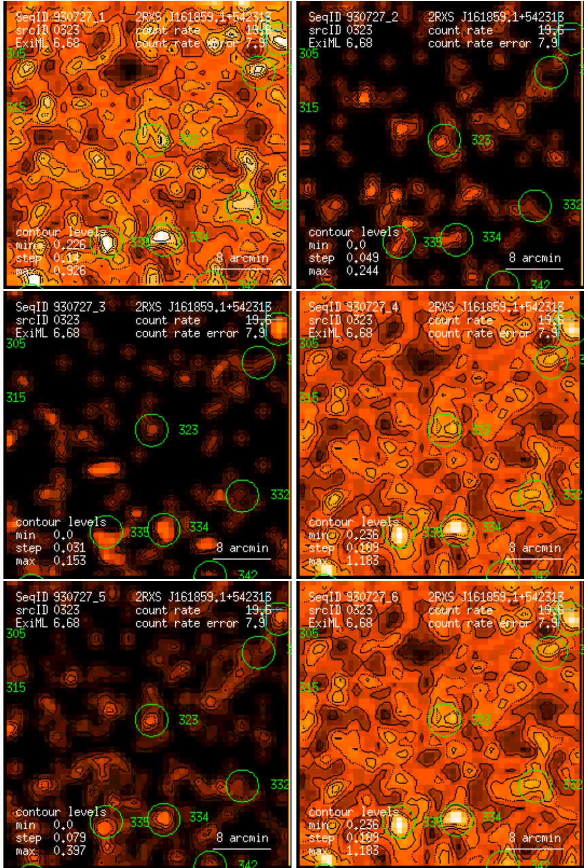
Figure 323: RASS 930727: detection 0323: band rate images, Gaussian filter: (1) PSPC channels 11 – 41, (2) 52 – 90, (3) 91 – 201, (4) 11 – 235, (5) 52 – 201, (6) 11 – 201. Broad band rates in counts/ks. Band rate contour levels in counts/ks/arcmin 2 .
