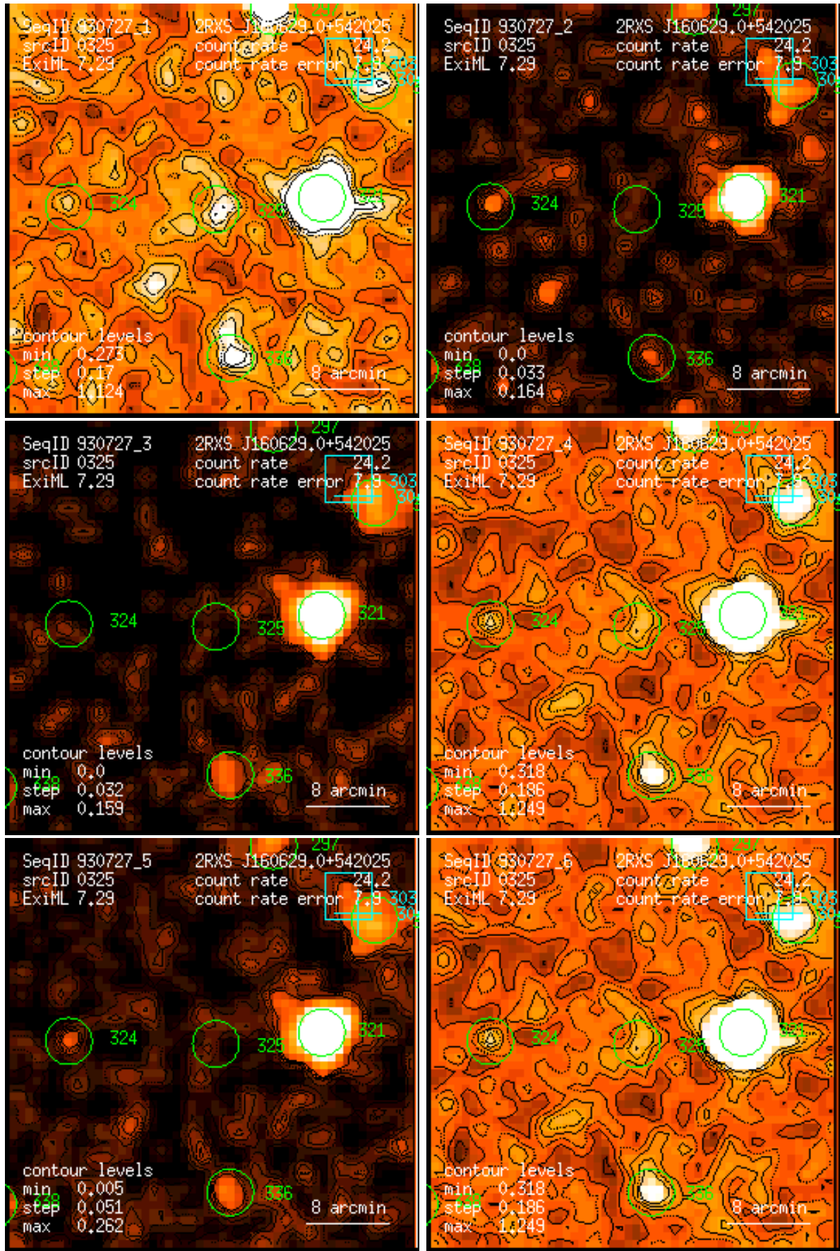
Figure 325: RASS 930727: detection 0325: band rate images, Gaussian filter: (1) PSPC channels 11 – 41, (2) 52 – 90, (3) 91 – 201, (4) 11 – 235, (5) 52 – 201, (6) 11 – 201. Broad band rates in counts/ks. Band rate contour levels in counts/ks/arcmin 2 .
