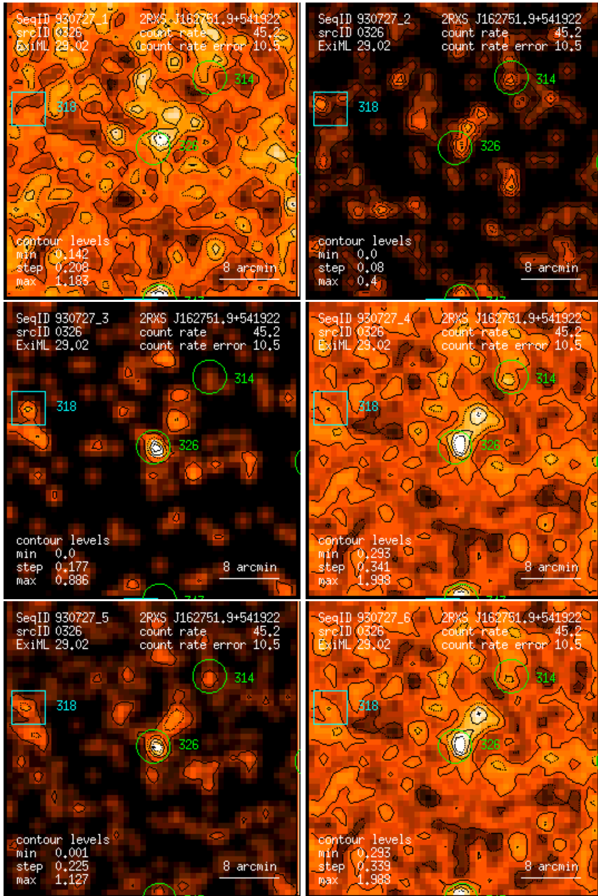
Figure 326: RASS 930727: detection 0326: band rate images, Gaussian filter: (1) PSPC channels 11 – 41, (2) 52 – 90, (3) 91 – 201, (4) 11 – 235, (5) 52 – 201, (6) 11 – 201. Broad band rates in counts/ks. Band rate contour levels in counts/ks/arcmin 2 .
