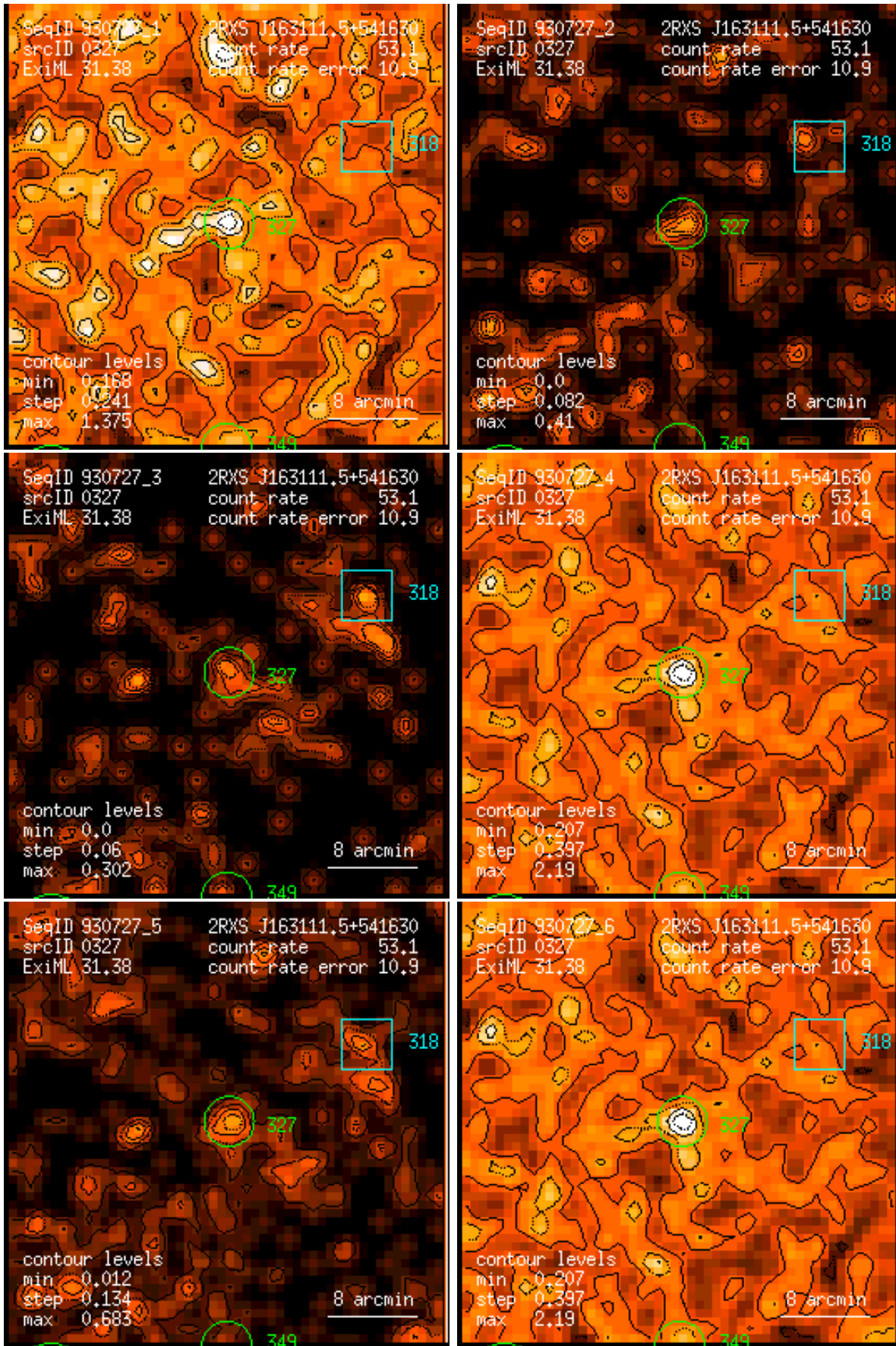
Figure 327: RASS 930727: detection 0327: band rate images, Gaussian filter: (1) PSPC channels 11 – 41, (2) 52 – 90, (3) 91 – 201, (4) 11 – 235, (5) 52 – 201, (6) 11 – 201. Broad band rates in counts/ks. Band rate contour levels in counts/ks/arcmin 2 .
