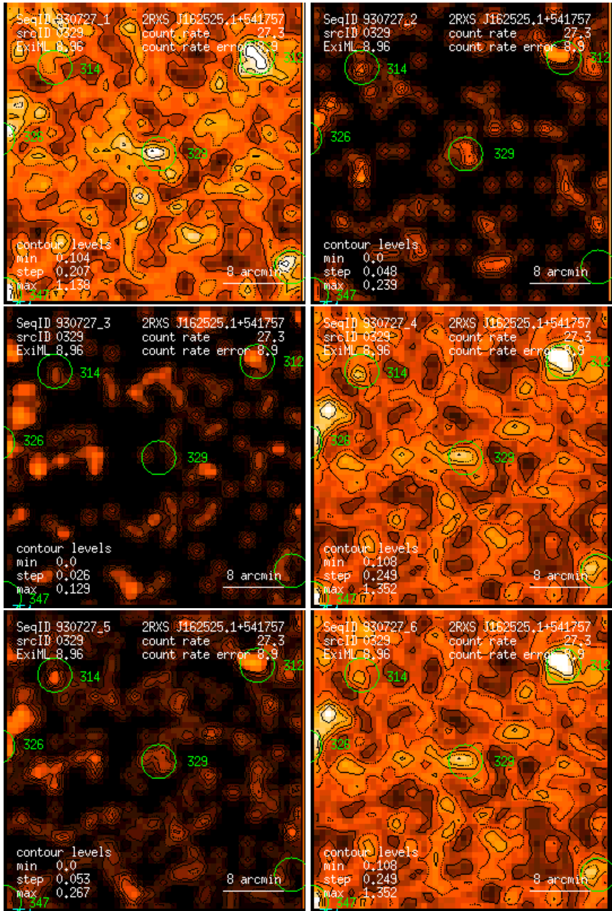
Figure 329: RASS 930727: detection 0329: band rate images, Gaussian filter: (1) PSPC channels 11 – 41, (2) 52 – 90, (3) 91 – 201, (4) 11 – 235, (5) 52 – 201, (6) 11 – 201. Broad band rates in counts/ks. Band rate contour levels in counts/ks/arcmin 2 .
