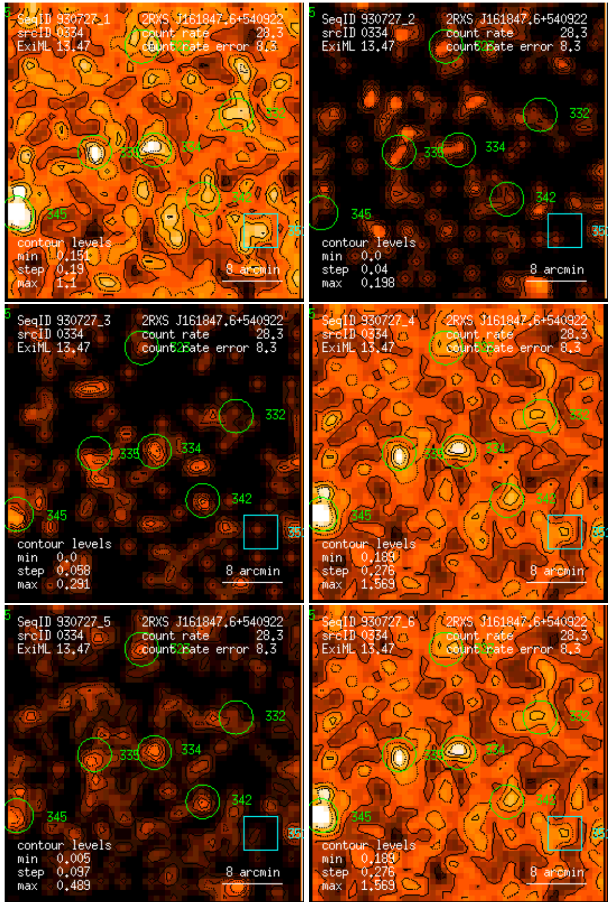
Figure 334: RASS 930727: detection 0334: band rate images, Gaussian filter: (1) PSPC channels 11 – 41, (2) 52 – 90, (3) 91 – 201, (4) 11 – 235, (5) 52 – 201, (6) 11 – 201. Broad band rates in counts/ks. Band rate contour levels in counts/ks/arcmin 2 .
