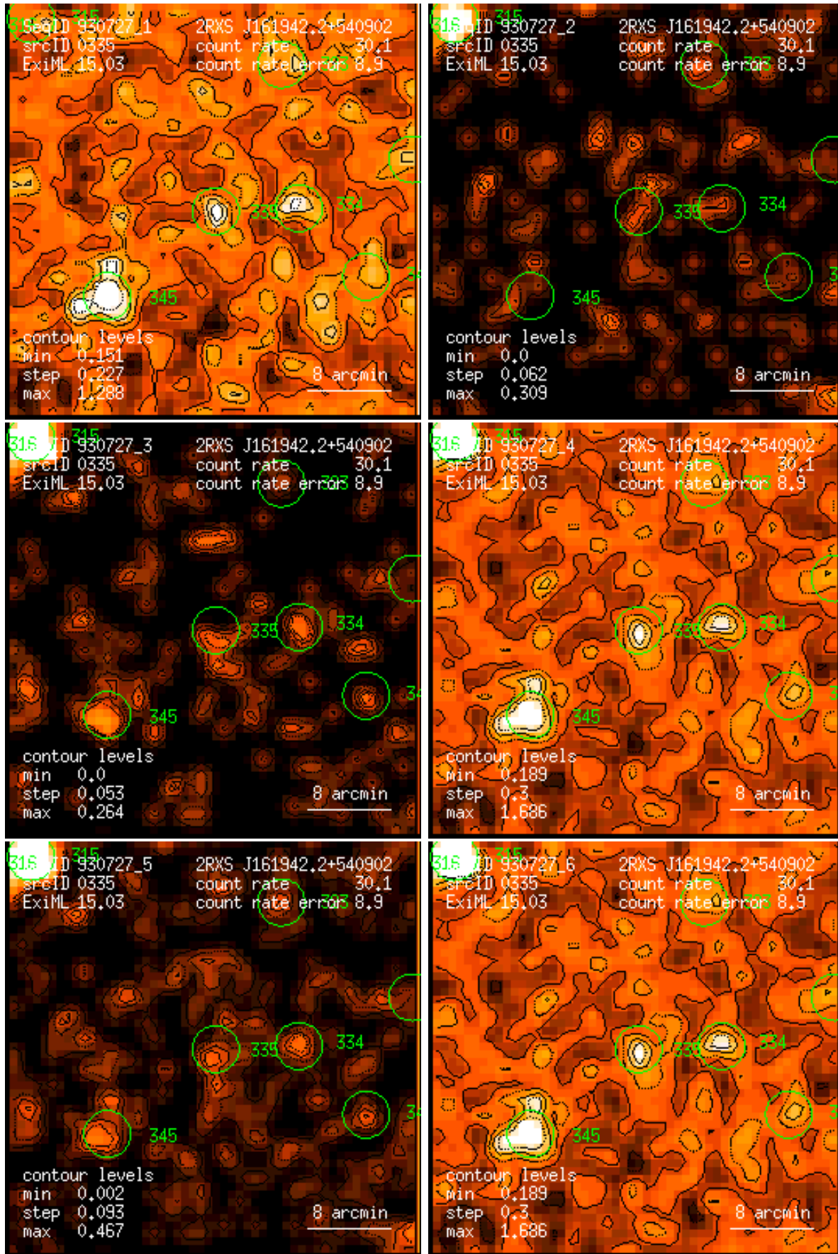
Figure 335: RASS 930727: detection 0335: band rate images, Gaussian filter: (1) PSPC channels 11 – 41, (2) 52 – 90, (3) 91 – 201, (4) 11 – 235, (5) 52 – 201, (6) 11 – 201. Broad band rates in counts/ks. Band rate contour levels in counts/ks/arcmin 2 .
