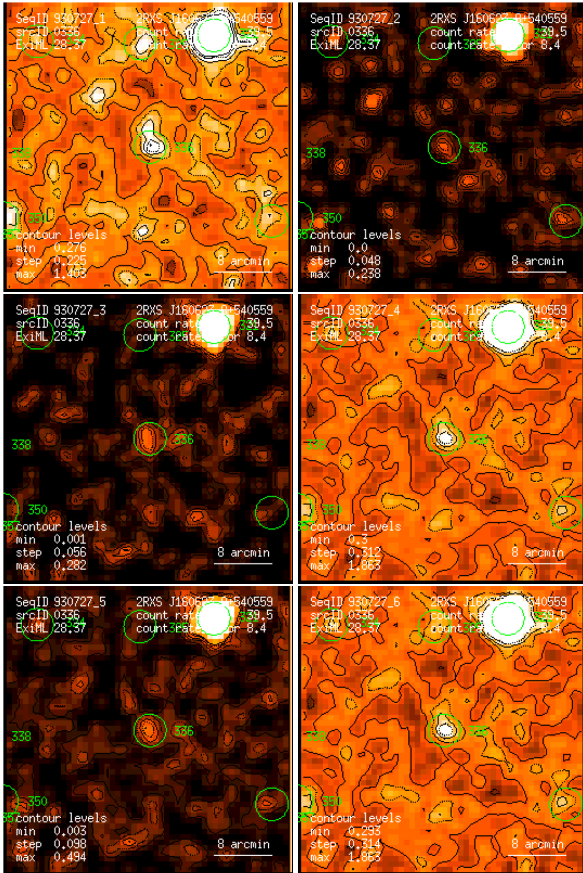
Figure 336: RASS 930727: detection 0336: band rate images, Gaussian filter: (1) PSPC channels 11 – 41, (2) 52 – 90, (3) 91 – 201, (4) 11 – 235, (5) 52 – 201, (6) 11 – 201. Broad band rates in counts/ks. Band rate contour levels in counts/ks/arcmin 2 .
