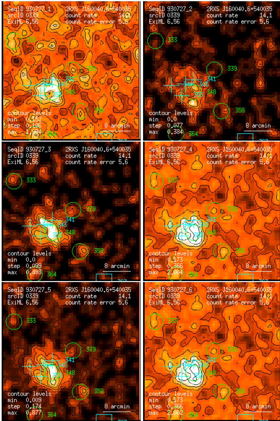
Figure 339: RASS 930727: detection 0339: band rate images, Gaussian filter: (1) PSPC channels 11 – 41, (2) 52 – 90, (3) 91 – 201, (4) 11 – 235, (5) 52 – 201, (6) 11 – 201. Broad band rates in counts/ks. Band rate contour levels in counts/ks/arcmin 2 .
