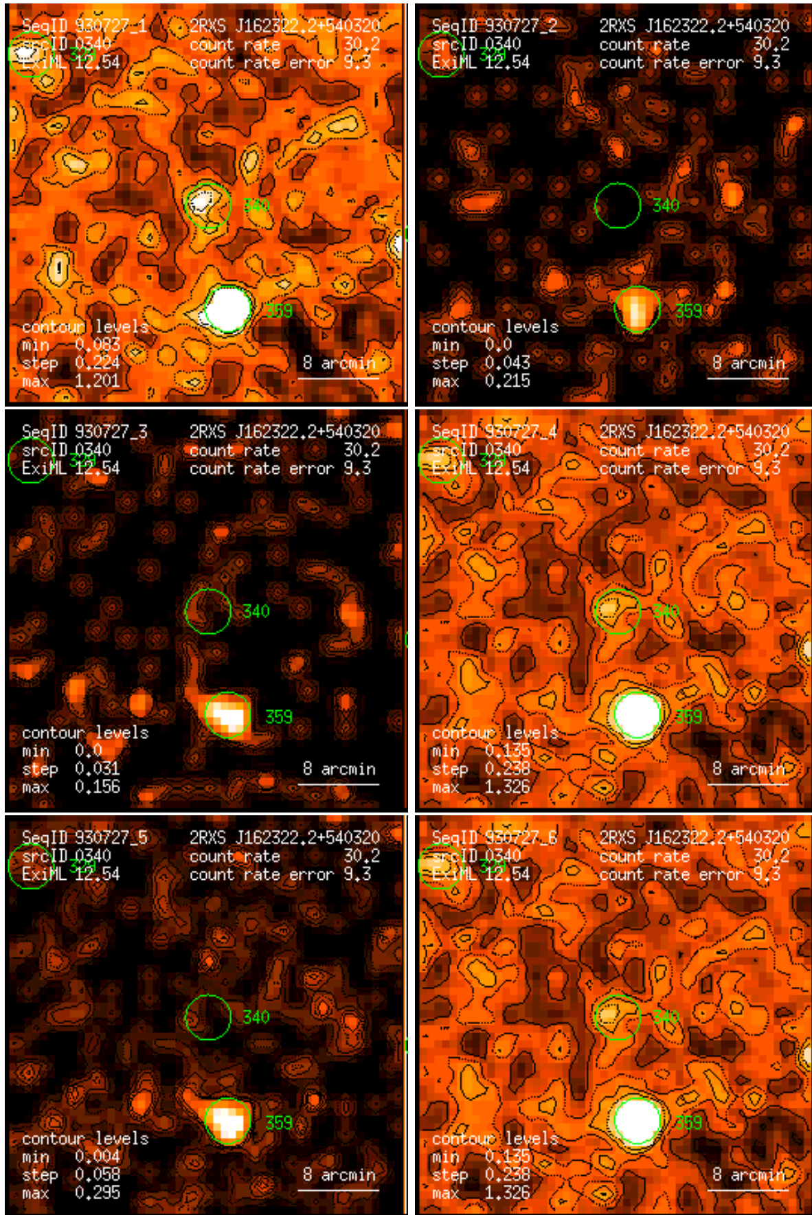
Figure 340: RASS 930727: detection 0340: band rate images, Gaussian filter: (1) PSPC channels 11 – 41, (2) 52 – 90, (3) 91 – 201, (4) 11 – 235, (5) 52 – 201, (6) 11 – 201. Broad band rates in counts/ks. Band rate contour levels in counts/ks/arcmin 2 .
