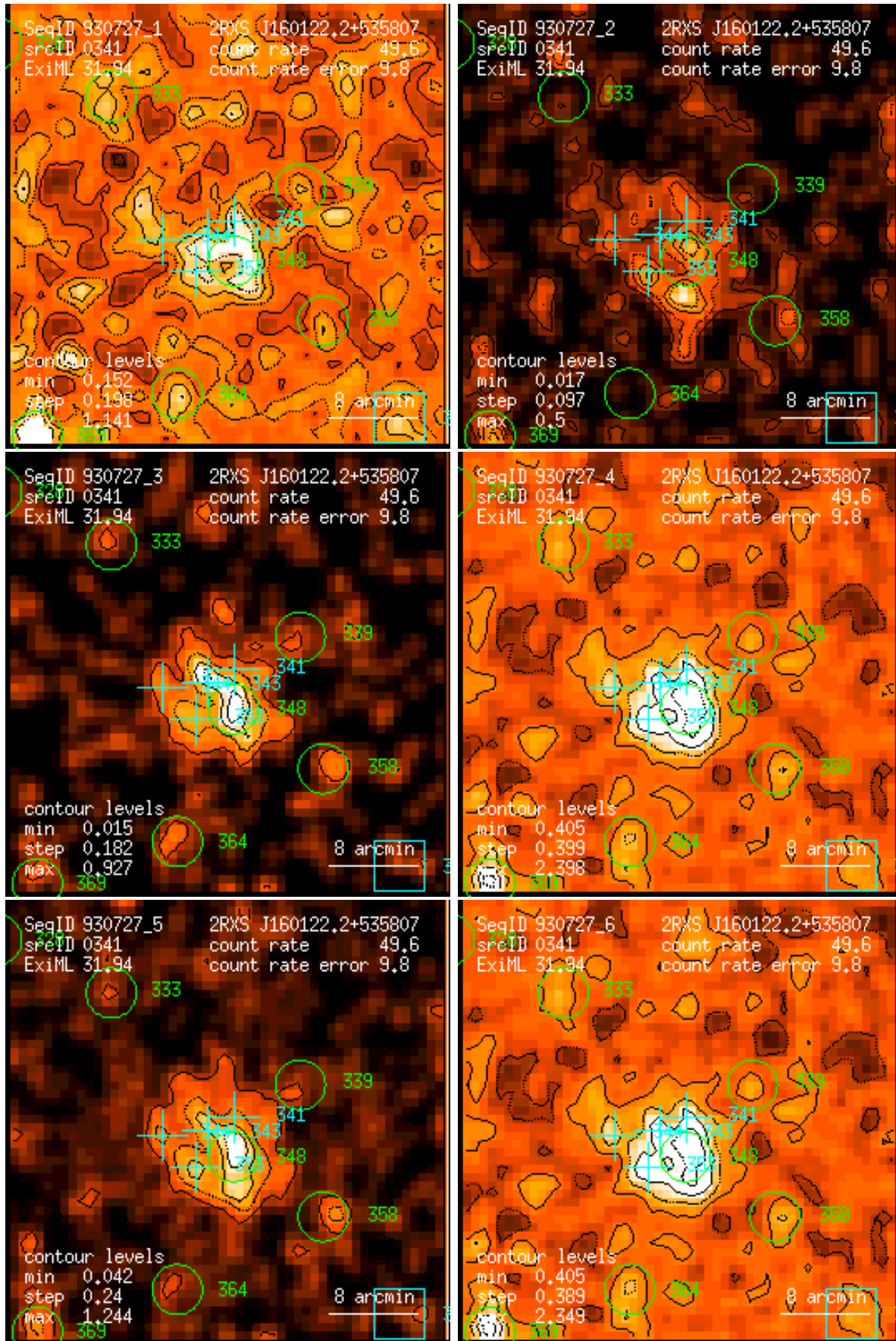
Figure 341: RASS 930727: detection 0341: band rate images, Gaussian filter: (1) PSPC channels 11 – 41, (2) 52 – 90, (3) 91 – 201, (4) 11 – 235, (5) 52 – 201, (6) 11 – 201. Broad band rates in counts/ks. Band rate contour levels in counts/ks/arcmin 2 .
