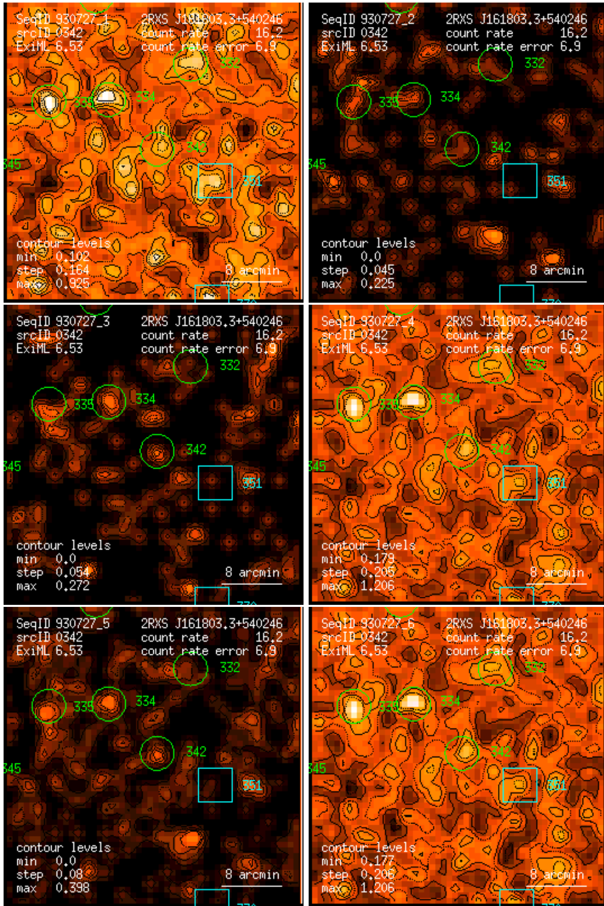
Figure 342: RASS 930727: detection 0342: band rate images, Gaussian filter: (1) PSPC channels 11 – 41, (2) 52 – 90, (3) 91 – 201, (4) 11 – 235, (5) 52 – 201, (6) 11 – 201. Broad band rates in counts/ks. Band rate contour levels in counts/ks/arcmin 2 .
