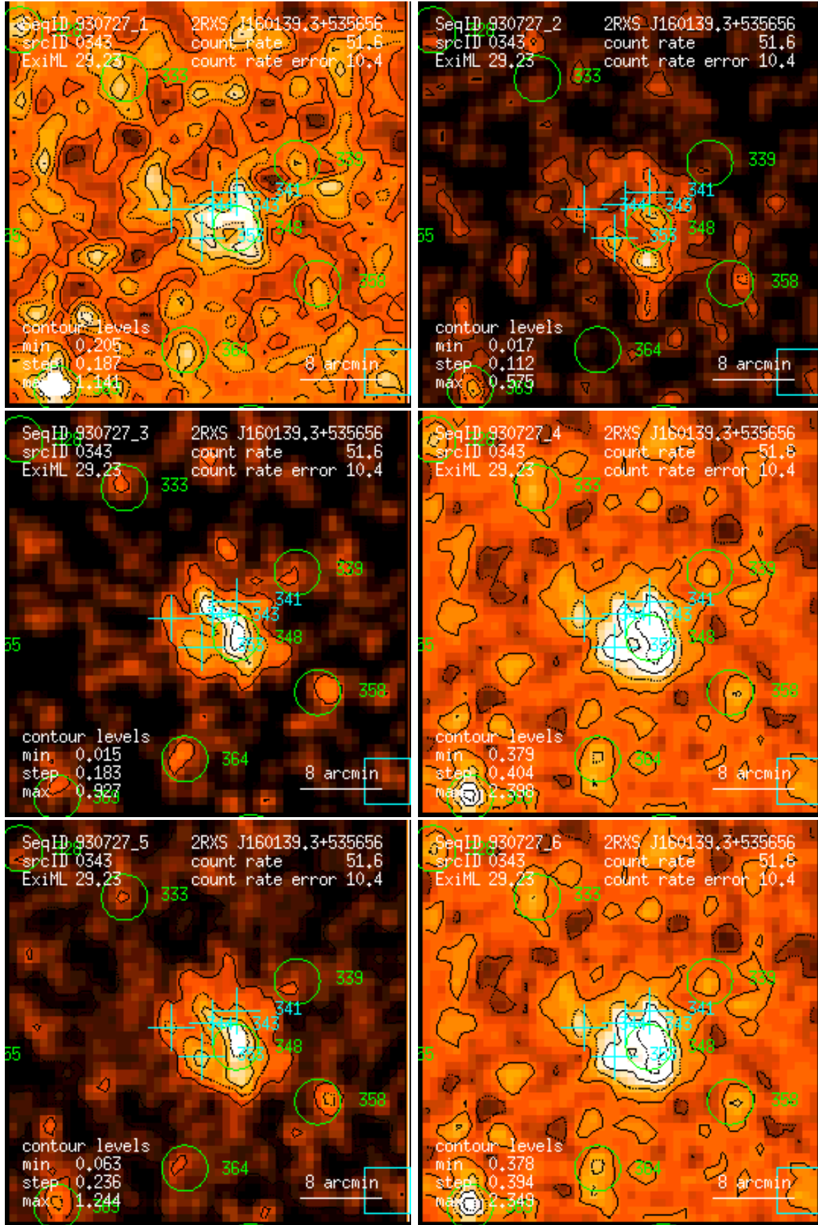
Figure 343: RASS 930727: detection 0343: band rate images, Gaussian filter: (1) PSPC channels 11 – 41, (2) 52 – 90, (3) 91 – 201, (4) 11 – 235, (5) 52 – 201, (6) 11 – 201. Broad band rates in counts/ks. Band rate contour levels in counts/ks/arcmin 2 .
