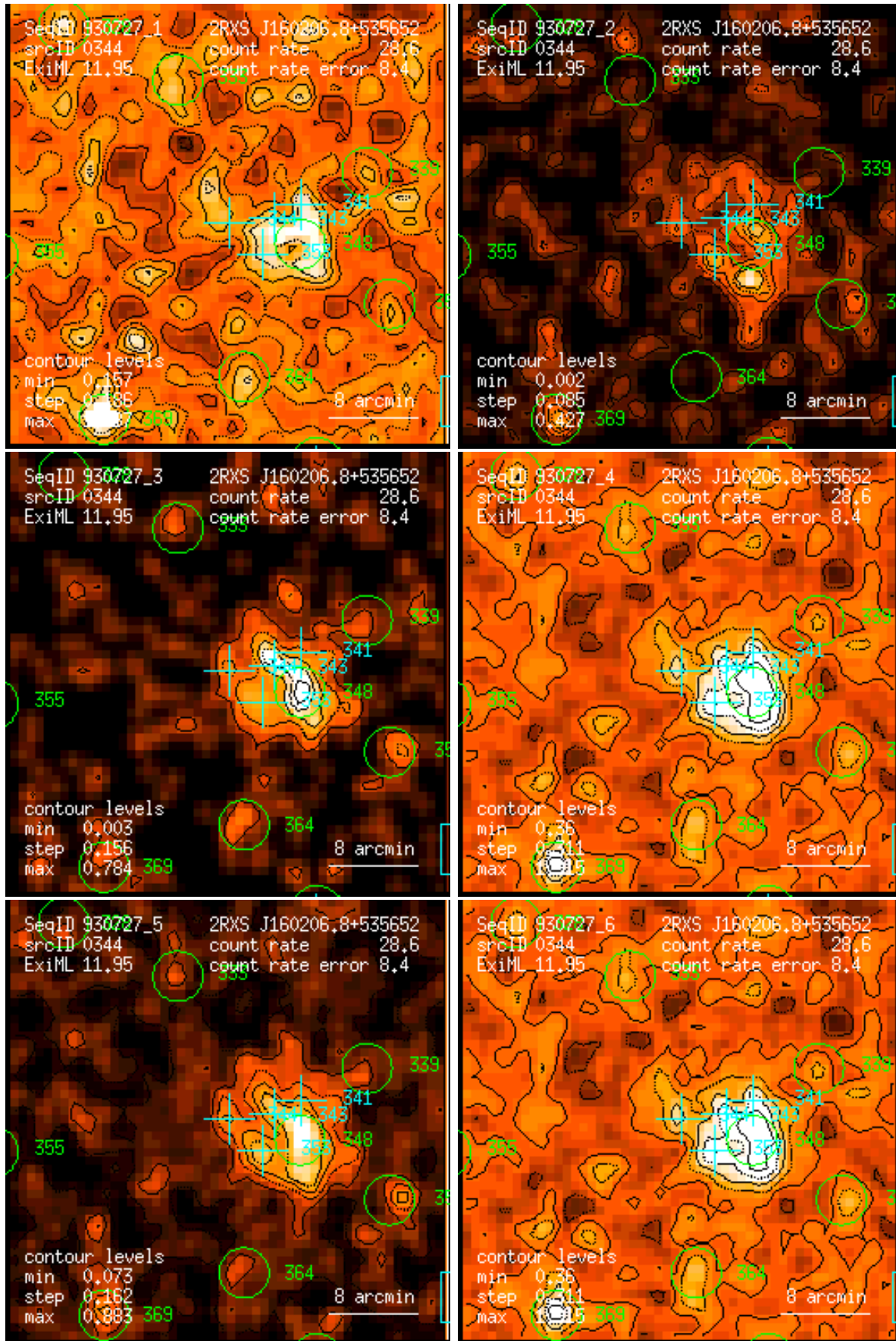
Figure 344: RASS 930727: detection 0344: band rate images, Gaussian filter: (1) PSPC channels 11 – 41, (2) 52 – 90, (3) 91 – 201, (4) 11 – 235, (5) 52 – 201, (6) 11 – 201. Broad band rates in counts/ks. Band rate contour levels in counts/ks/arcmin 2 .
