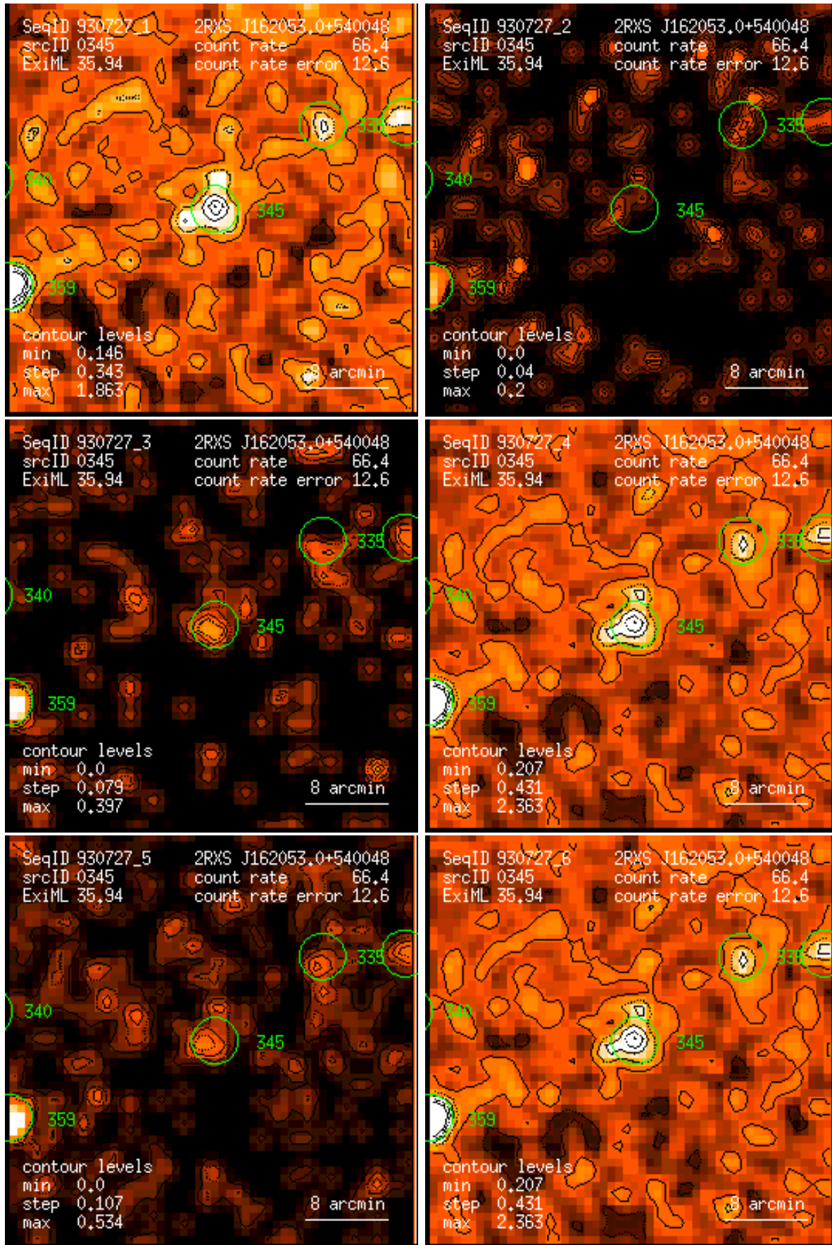
Figure 345: RASS 930727: detection 0345: band rate images, Gaussian filter: (1) PSPC channels 11 – 41, (2) 52 – 90, (3) 91 – 201, (4) 11 – 235, (5) 52 – 201, (6) 11 – 201. Broad band rates in counts/ks. Band rate contour levels in counts/ks/arcmin 2 .
