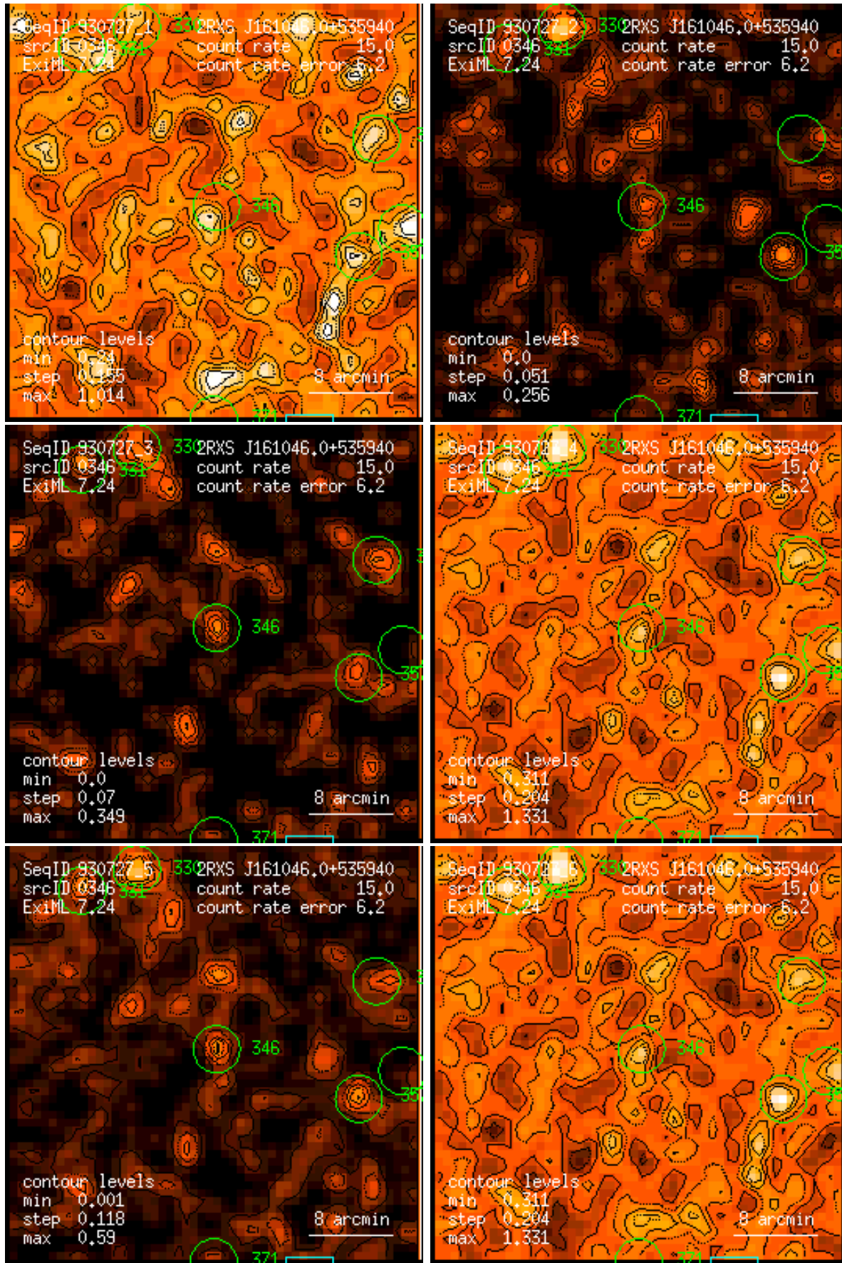
Figure 346: RASS 930727: detection 0346: band rate images, Gaussian filter: (1) PSPC channels 11 – 41, (2) 52 – 90, (3) 91 – 201, (4) 11 – 235, (5) 52 – 201, (6) 11 – 201. Broad band rates in counts/ks. Band rate contour levels in counts/ks/arcmin 2 .
