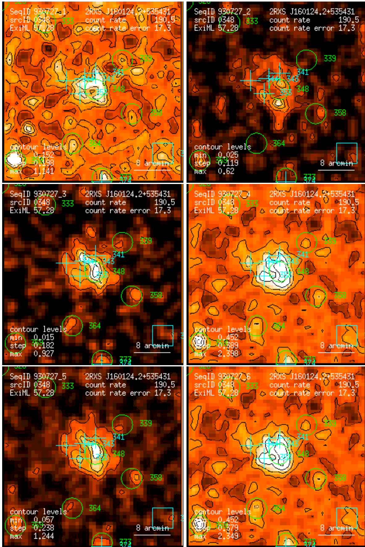
Figure 348: RASS 930727: detection 0348: band rate images, Gaussian filter: (1) PSPC channels 11 – 41, (2) 52 – 90, (3) 91 – 201, (4) 11 – 235, (5) 52 – 201, (6) 11 – 201. Broad band rates in counts/ks. Band rate contour levels in counts/ks/arcmin 2 .
