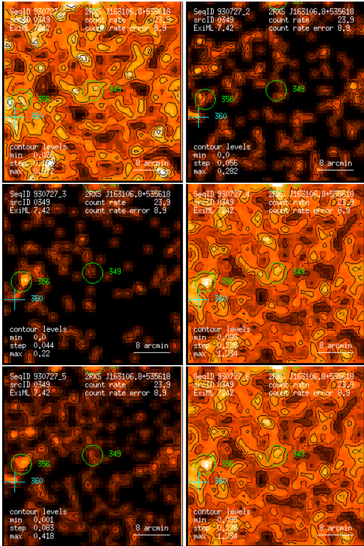
Figure 349: RASS 930727: detection 0349: band rate images, Gaussian filter: (1) PSPC channels 11 – 41, (2) 52 – 90, (3) 91 – 201, (4) 11 – 235, (5) 52 – 201, (6) 11 – 201. Broad band rates in counts/ks. Band rate contour levels in counts/ks/arcmin 2 .
