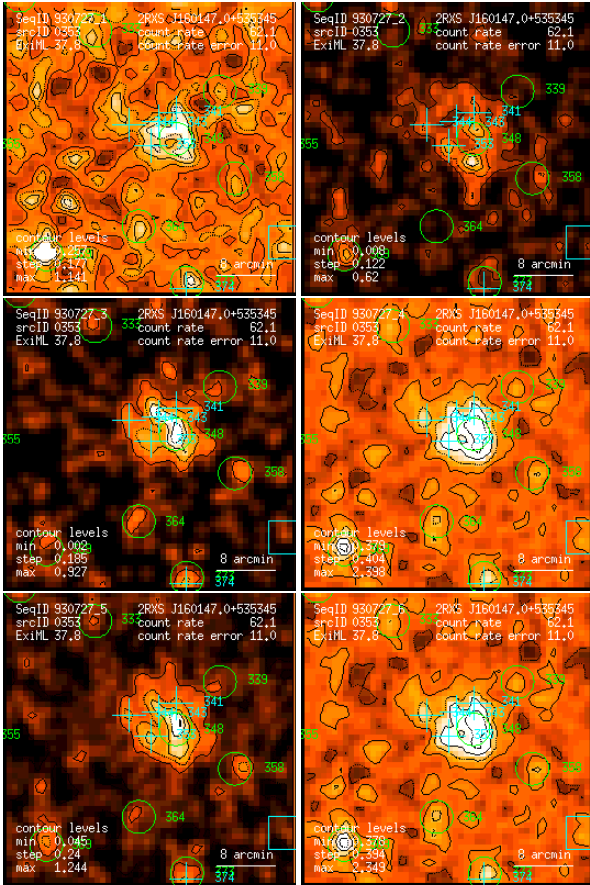
Figure 353: RASS 930727: detection 0353: band rate images, Gaussian filter: (1) PSPC channels 11 – 41, (2) 52 – 90, (3) 91 – 201, (4) 11 – 235, (5) 52 – 201, (6) 11 – 201. Broad band rates in counts/ks. Band rate contour levels in counts/ks/arcmin 2 .
