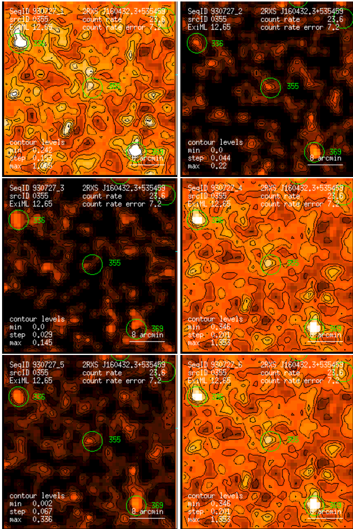
Figure 355: RASS 930727: detection 0355: band rate images, Gaussian filter: (1) PSPC channels 11 – 41, (2) 52 – 90, (3) 91 – 201, (4) 11 – 235, (5) 52 – 201, (6) 11 – 201. Broad band rates in counts/ks. Band rate contour levels in counts/ks/arcmin 2 .
