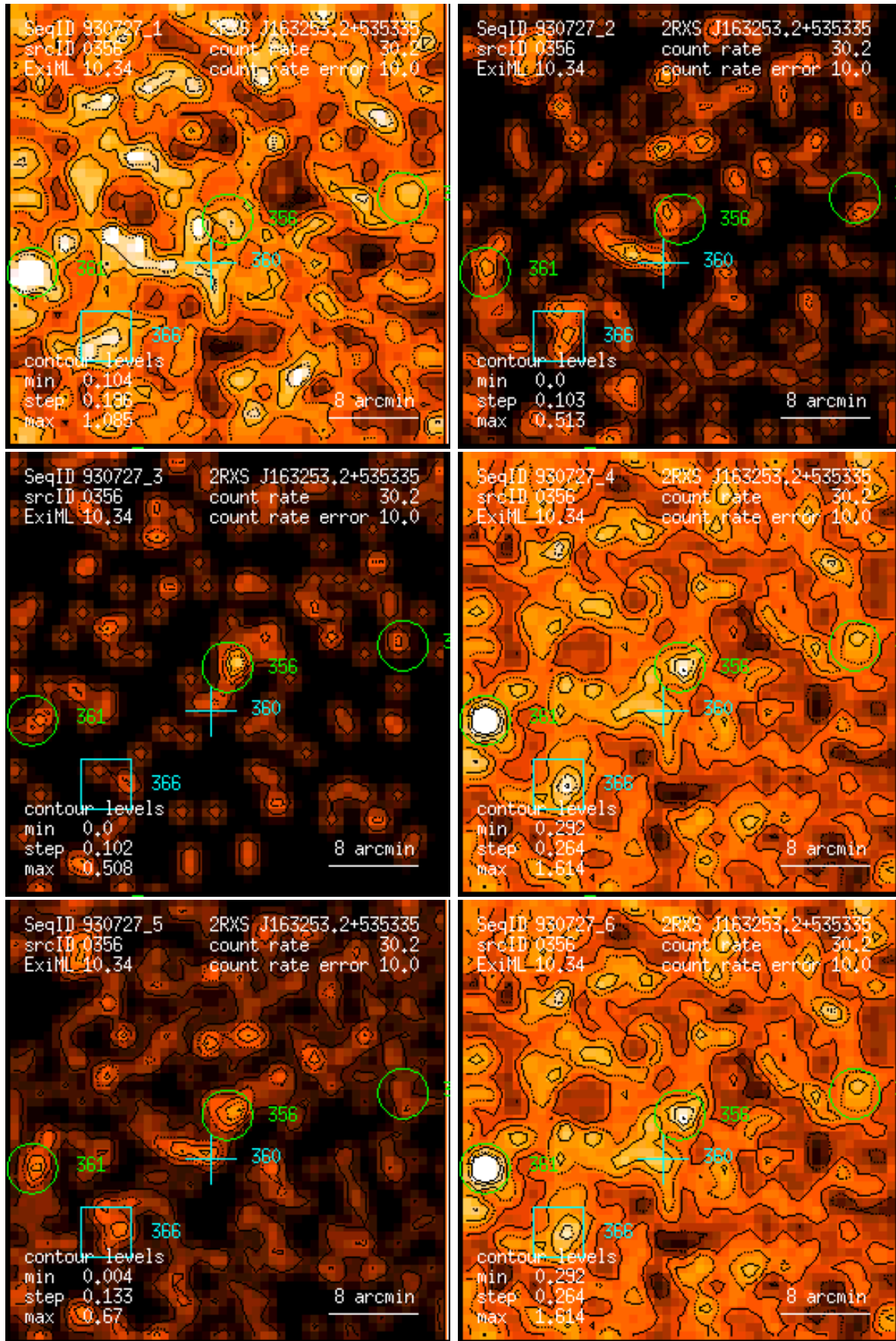
Figure 356: RASS 930727: detection 0356: band rate images, Gaussian filter: (1) PSPC channels 11 – 41, (2) 52 – 90, (3) 91 – 201, (4) 11 – 235, (5) 52 – 201, (6) 11 – 201. Broad band rates in counts/ks. Band rate contour levels in counts/ks/arcmin 2 .
