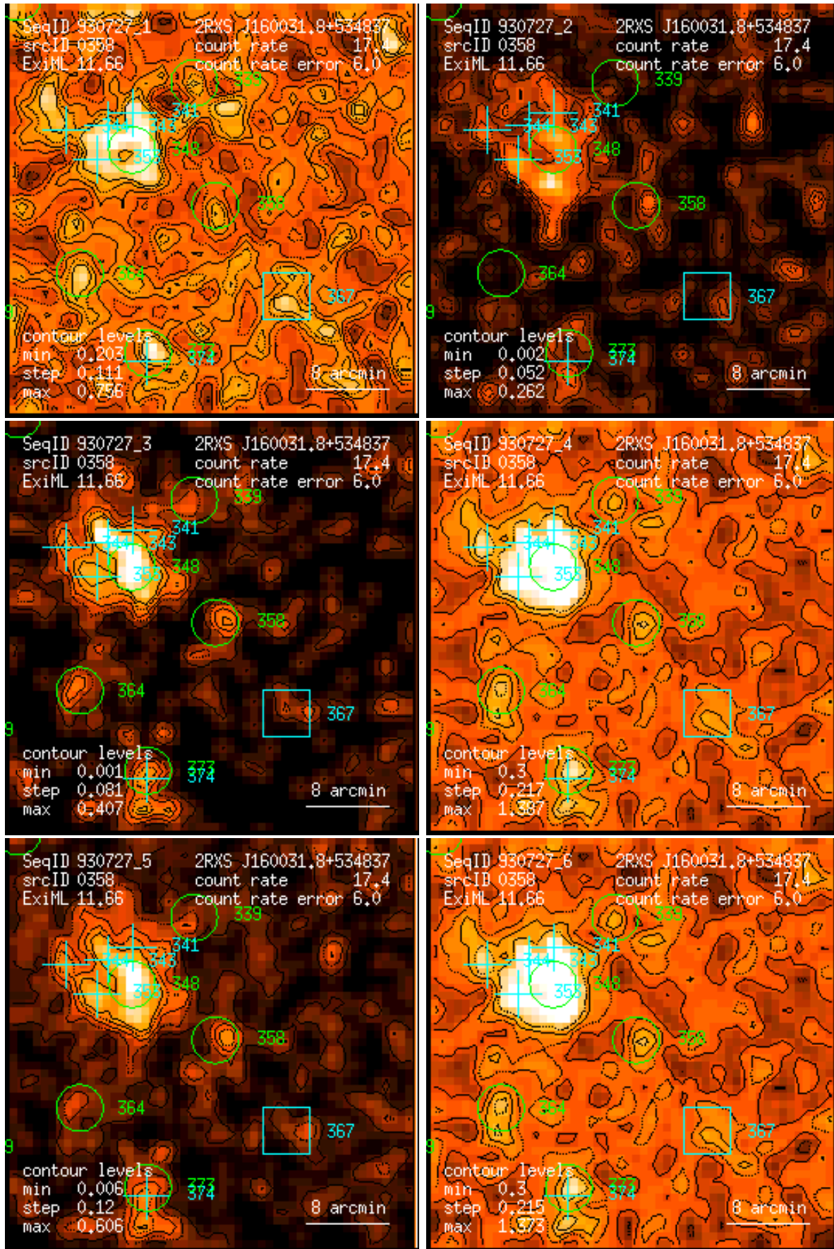
Figure 358: RASS 930727: detection 0358: band rate images, Gaussian filter: (1) PSPC channels 11 – 41, (2) 52 – 90, (3) 91 – 201, (4) 11 – 235, (5) 52 – 201, (6) 11 – 201. Broad band rates in counts/ks. Band rate contour levels in counts/ks/arcmin 2 .
