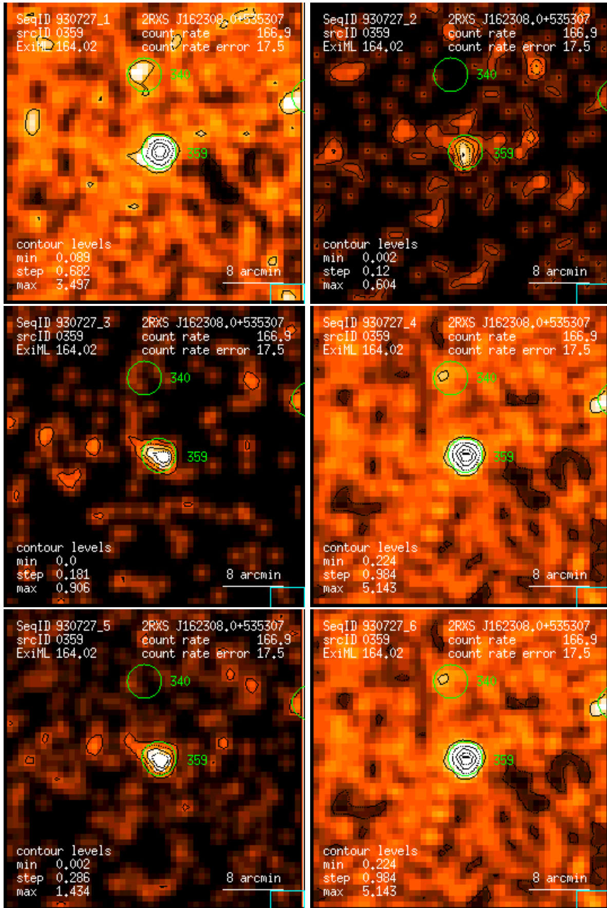
Figure 359: RASS 930727: detection 0359: band rate images, Gaussian filter: (1) PSPC channels 11 – 41, (2) 52 – 90, (3) 91 – 201, (4) 11 – 235, (5) 52 – 201, (6) 11 – 201. Broad band rates in counts/ks. Band rate contour levels in counts/ks/arcmin 2 .
