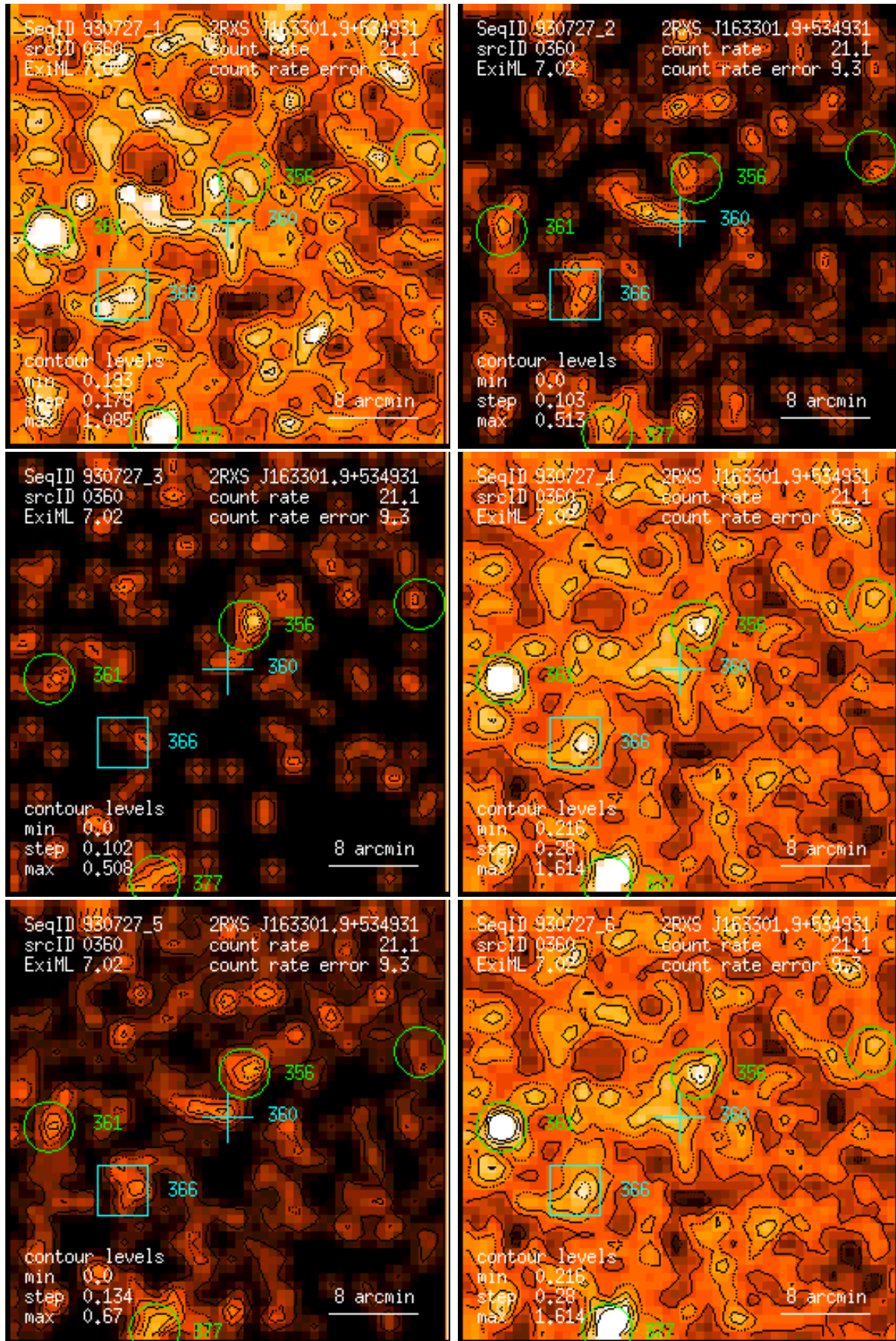
Figure 360: RASS 930727: detection 0360: band rate images, Gaussian filter: (1) PSPC channels 11 – 41, (2) 52 – 90, (3) 91 – 201, (4) 11 – 235, (5) 52 – 201, (6) 11 – 201. Broad band rates in counts/ks. Band rate contour levels in counts/ks/arcmin 2 .
