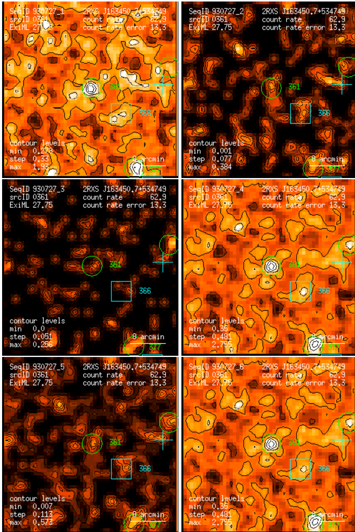
Figure 361: RASS 930727: detection 0361: band rate images, Gaussian filter: (1) PSPC channels 11 – 41, (2) 52 – 90, (3) 91 – 201, (4) 11 – 235, (5) 52 – 201, (6) 11 – 201. Broad band rates in counts/ks. Band rate contour levels in counts/ks/arcmin 2 .
