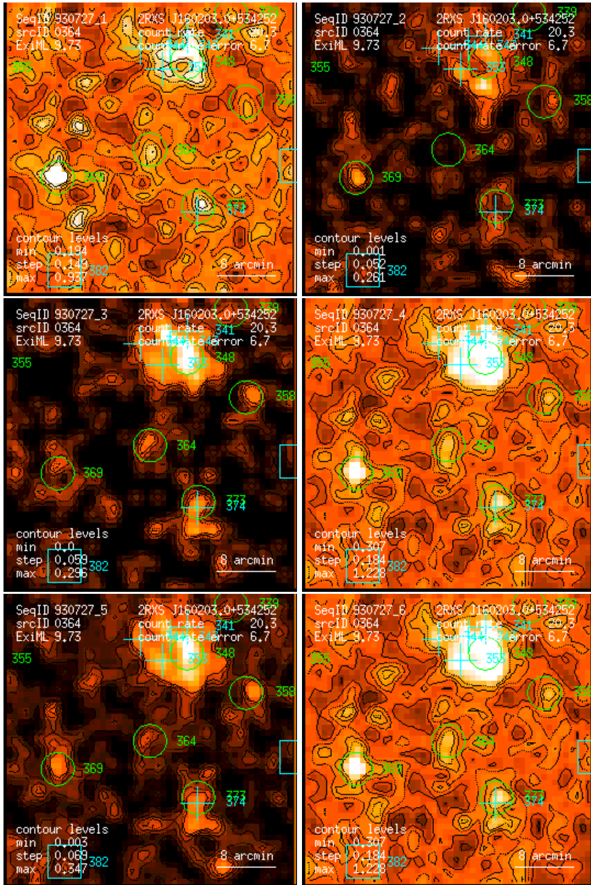
Figure 364: RASS 930727: detection 0364: band rate images, Gaussian filter: (1) PSPC channels 11 – 41, (2) 52 – 90, (3) 91 – 201, (4) 11 – 235, (5) 52 – 201, (6) 11 – 201. Broad band rates in counts/ks. Band rate contour levels in counts/ks/arcmin 2 .
