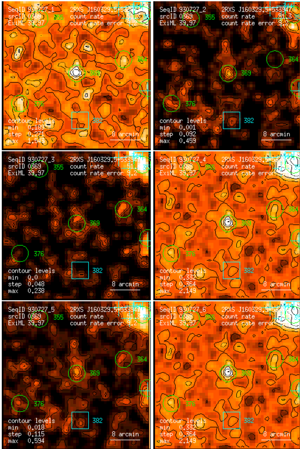
Figure 369: RASS 930727: detection 0369: band rate images, Gaussian filter: (1) PSPC channels 11 – 41, (2) 52 – 90, (3) 91 – 201, (4) 11 – 235, (5) 52 – 201, (6) 11 – 201. Broad band rates in counts/ks. Band rate contour levels in counts/ks/arcmin 2 .
