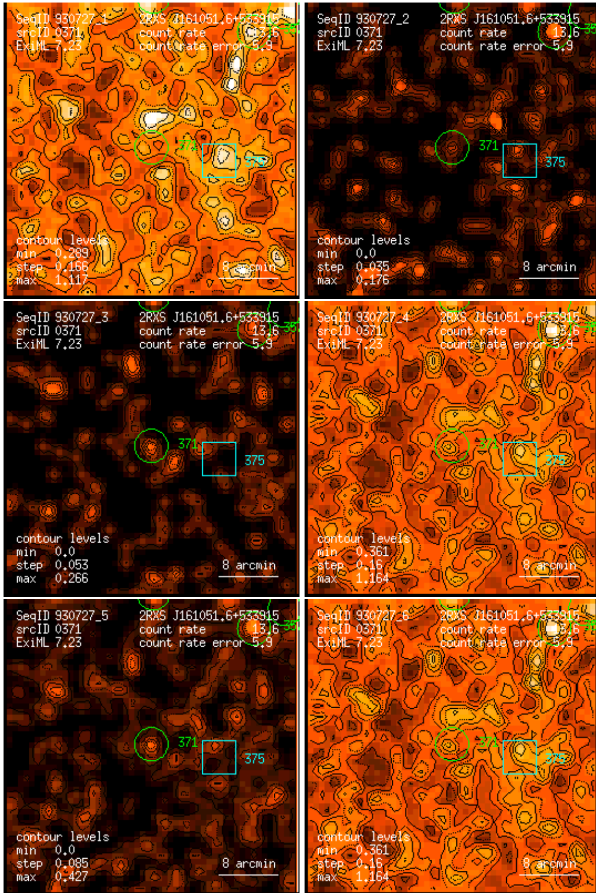
Figure 371: RASS 930727: detection 0371: band rate images, Gaussian filter: (1) PSPC channels 11 – 41, (2) 52 – 90, (3) 91 – 201, (4) 11 – 235, (5) 52 – 201, (6) 11 – 201. Broad band rates in counts/ks. Band rate contour levels in counts/ks/arcmin 2 .
