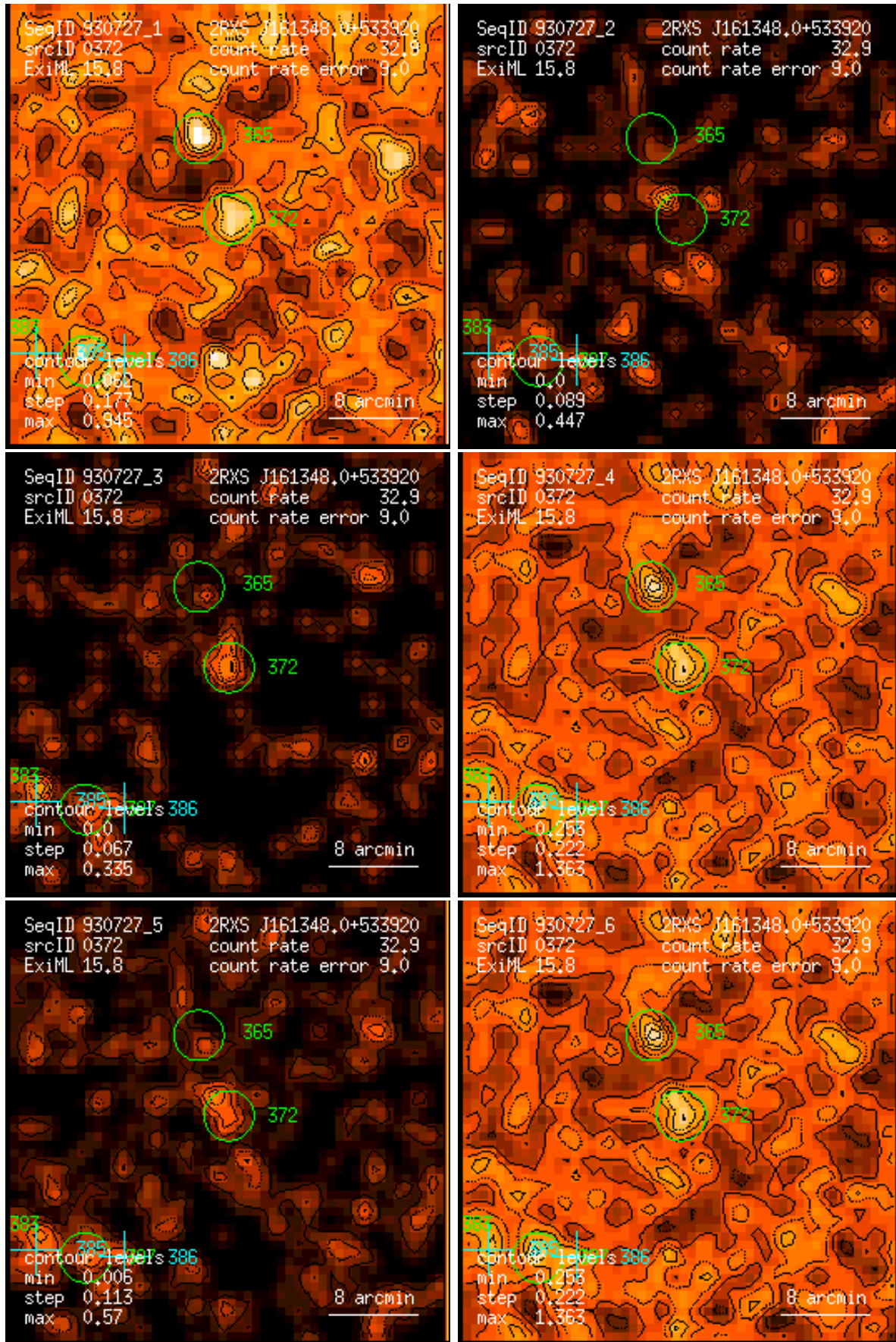
Figure 372: RASS 930727: detection 0372: band rate images, Gaussian filter: (1) PSPC channels 11 – 41, (2) 52 – 90, (3) 91 – 201, (4) 11 – 235, (5) 52 – 201, (6) 11 – 201. Broad band rates in counts/ks. Band rate contour levels in counts/ks/arcmin 2 .
