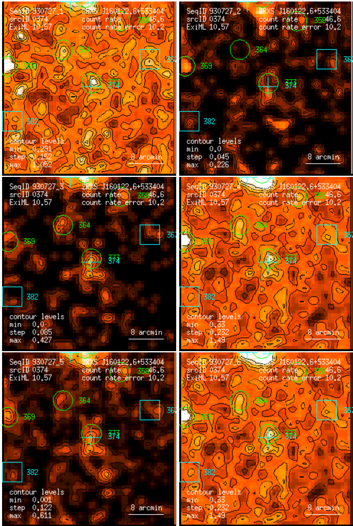
Figure 374: RASS 930727: detection 0374: band rate images, Gaussian filter: (1) PSPC channels 11 – 41, (2) 52 – 90, (3) 91 – 201, (4) 11 – 235, (5) 52 – 201, (6) 11 – 201. Broad band rates in counts/ks. Band rate contour levels in counts/ks/arcmin 2 .
