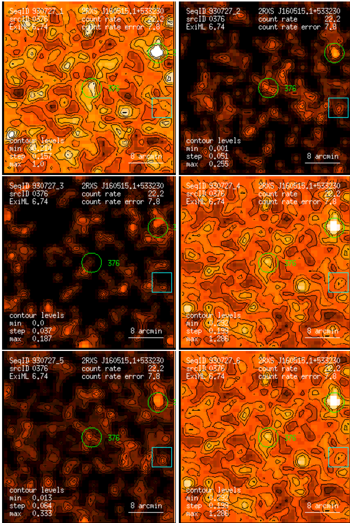
Figure 376: RASS 930727: detection 0376: band rate images, Gaussian filter: (1) PSPC channels 11 – 41, (2) 52 – 90, (3) 91 – 201, (4) 11 – 235, (5) 52 – 201, (6) 11 – 201. Broad band rates in counts/ks. Band rate contour levels in counts/ks/arcmin 2 .
