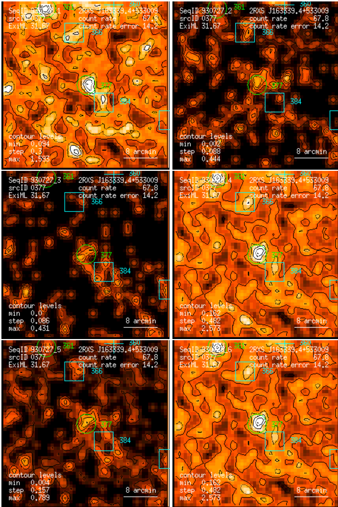
Figure 377: RASS 930727: detection 0377: band rate images, Gaussian filter: (1) PSPC channels 11 – 41, (2) 52 – 90, (3) 91 – 201, (4) 11 – 235, (5) 52 – 201, (6) 11 – 201. Broad band rates in counts/ks. Band rate contour levels in counts/ks/arcmin 2 .
