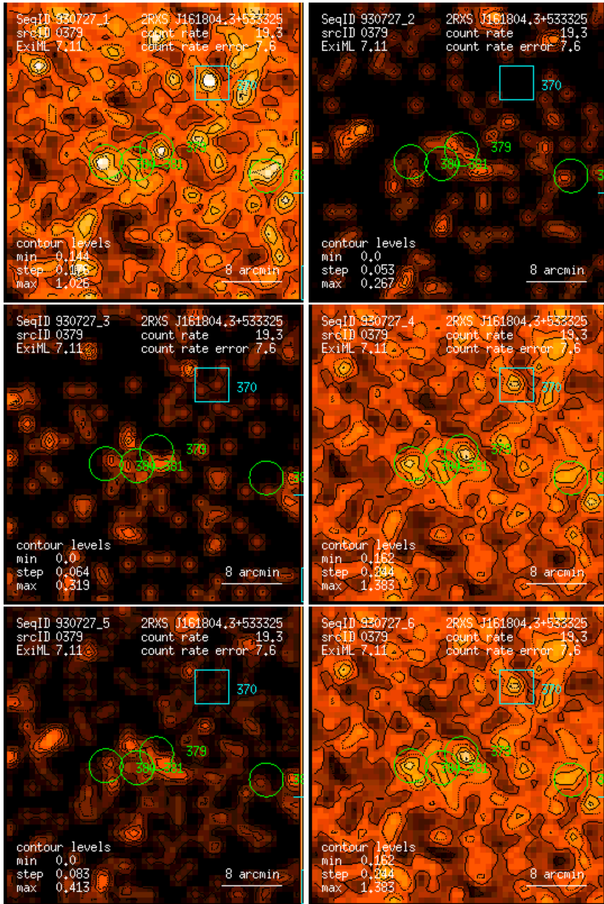
Figure 379: RASS 930727: detection 0379: band rate images, Gaussian filter: (1) PSPC channels 11 – 41, (2) 52 – 90, (3) 91 – 201, (4) 11 – 235, (5) 52 – 201, (6) 11 – 201. Broad band rates in counts/ks. Band rate contour levels in counts/ks/arcmin 2 .
