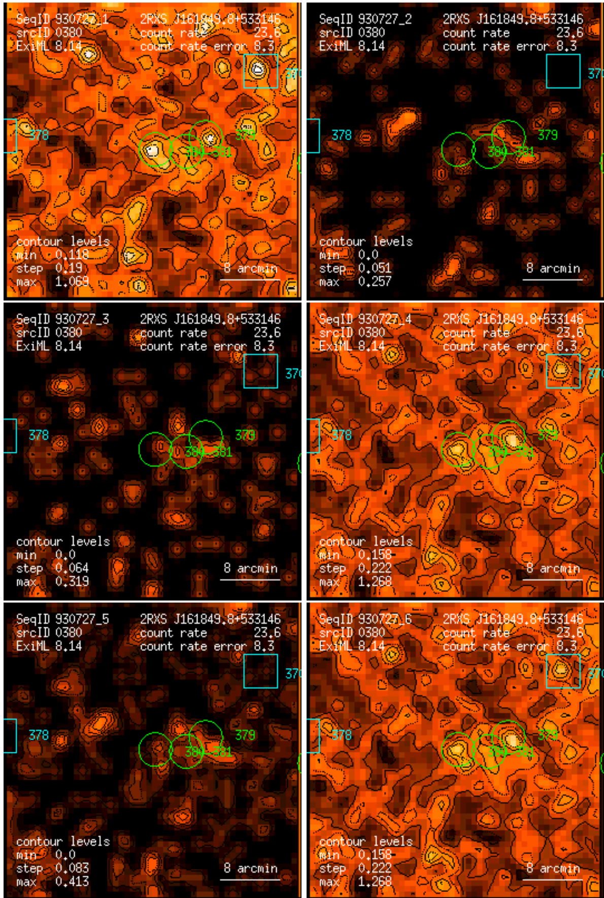
Figure 380: RASS 930727: detection 0380: band rate images, Gaussian filter: (1) PSPC channels 11 – 41, (2) 52 – 90, (3) 91 – 201, (4) 11 – 235, (5) 52 – 201, (6) 11 – 201. Broad band rates in counts/ks. Band rate contour levels in counts/ks/arcmin 2 .
