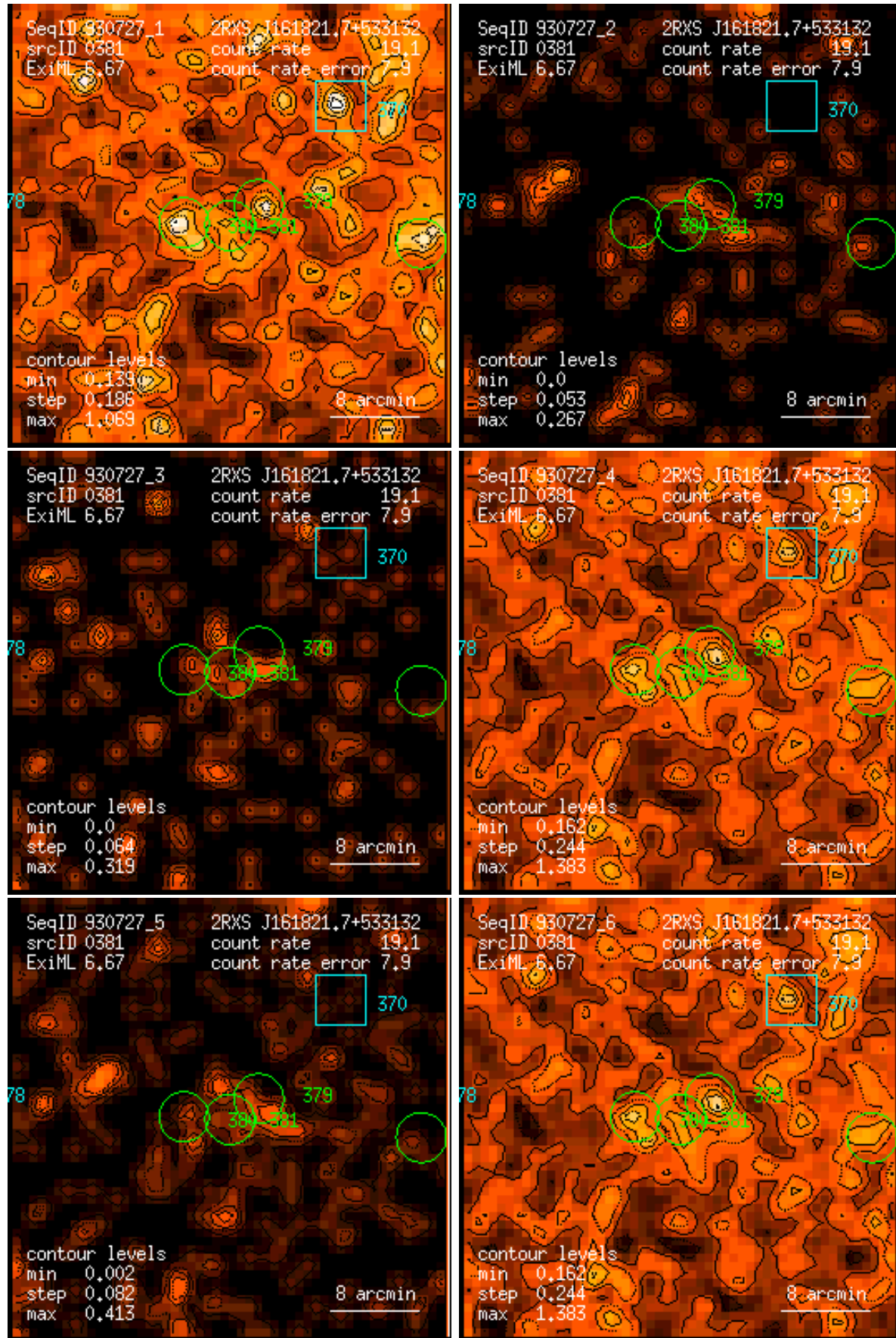
Figure 381: RASS 930727: detection 0381: band rate images, Gaussian filter: (1) PSPC channels 11 – 41, (2) 52 – 90, (3) 91 – 201, (4) 11 – 235, (5) 52 – 201, (6) 11 – 201. Broad band rates in counts/ks. Band rate contour levels in counts/ks/arcmin 2 .
