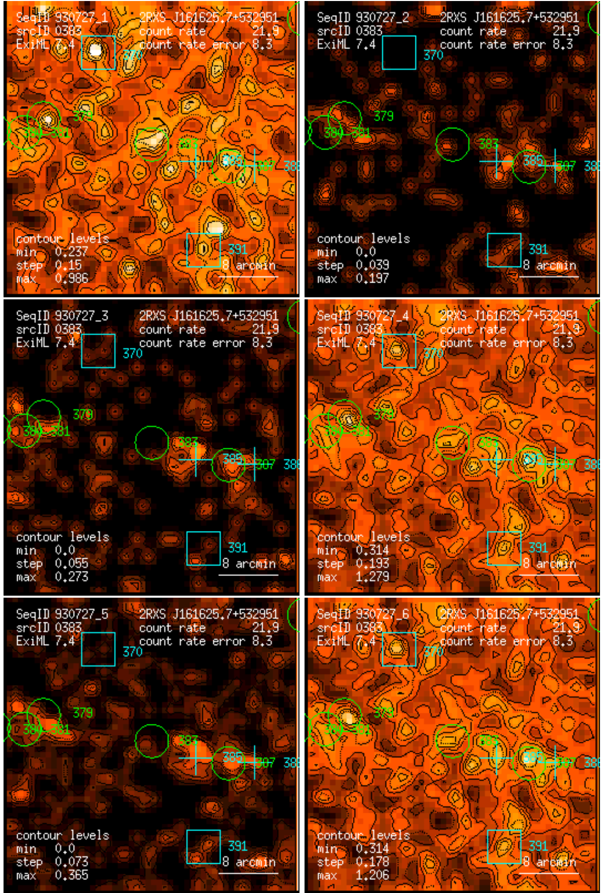
Figure 383: RASS 930727: detection 0383: band rate images, Gaussian filter: (1) PSPC channels 11 – 41, (2) 52 – 90, (3) 91 – 201, (4) 11 – 235, (5) 52 – 201, (6) 11 – 201. Broad band rates in counts/ks. Band rate contour levels in counts/ks/arcmin 2 .
