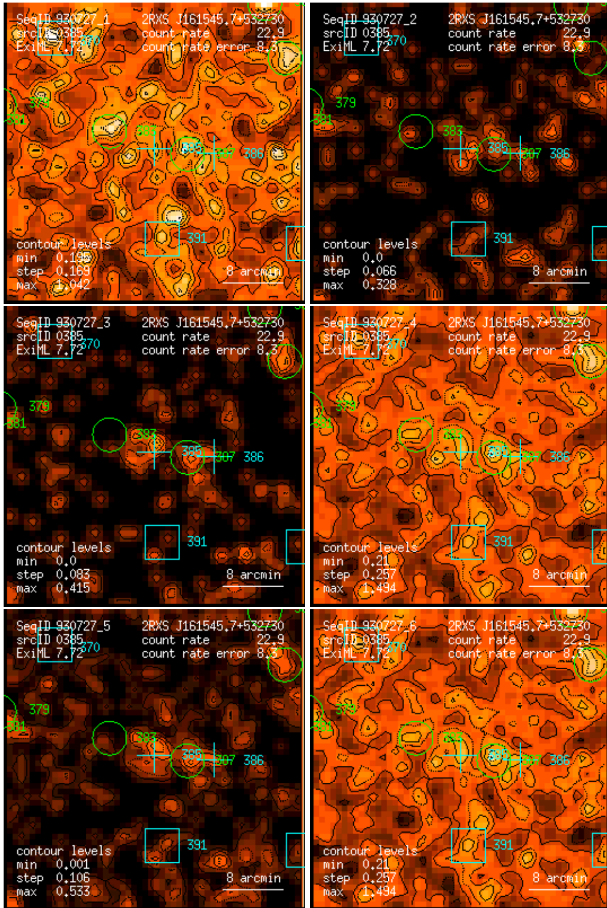
Figure 385: RASS 930727: detection 0385: band rate images, Gaussian filter: (1) PSPC channels 11 – 41, (2) 52 – 90, (3) 91 – 201, (4) 11 – 235, (5) 52 – 201, (6) 11 – 201. Broad band rates in counts/ks. Band rate contour levels in counts/ks/arcmin 2 .
