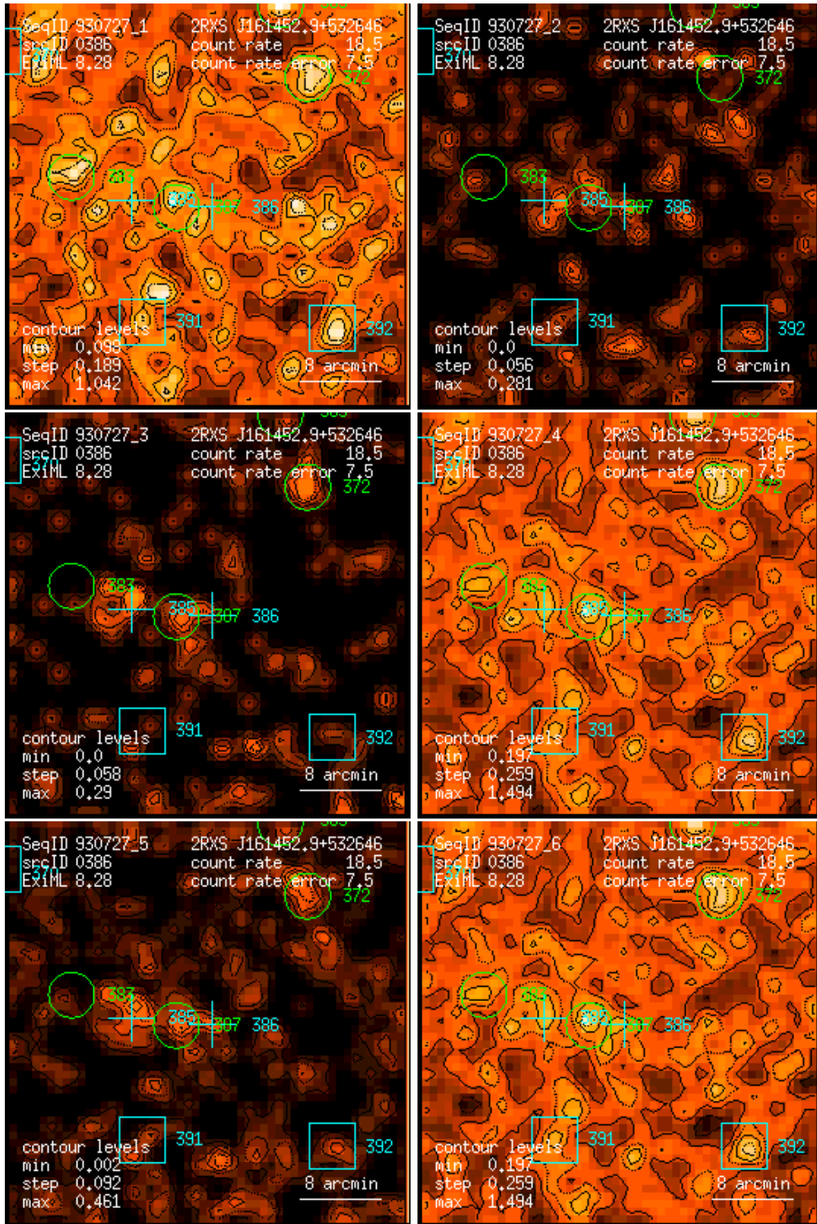
Figure 386: RASS 930727: detection 0386: band rate images, Gaussian filter: (1) PSPC channels 11 – 41, (2) 52 – 90, (3) 91 – 201, (4) 11 – 235, (5) 52 – 201, (6) 11 – 201. Broad band rates in counts/ks. Band rate contour levels in counts/ks/arcmin 2 .
