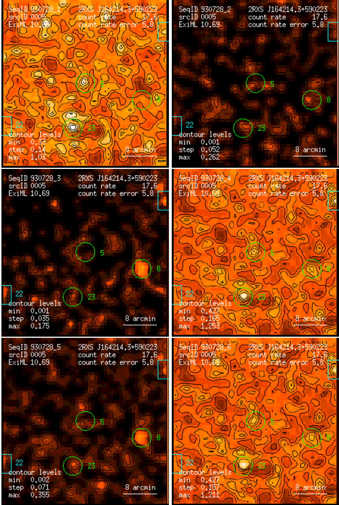
Figure 5: RASS 930728: detection 0005: band rate images, Gaussian filter: (1) PSPC channels 11 – 41, (2) 52 – 90, (3) 91 – 201, (4) 11 – 235, (5) 52 – 201, (6) 11 – 201. Broad band rates in counts/ks. Band rate contour levels in counts/ks/arcmin 2 .
