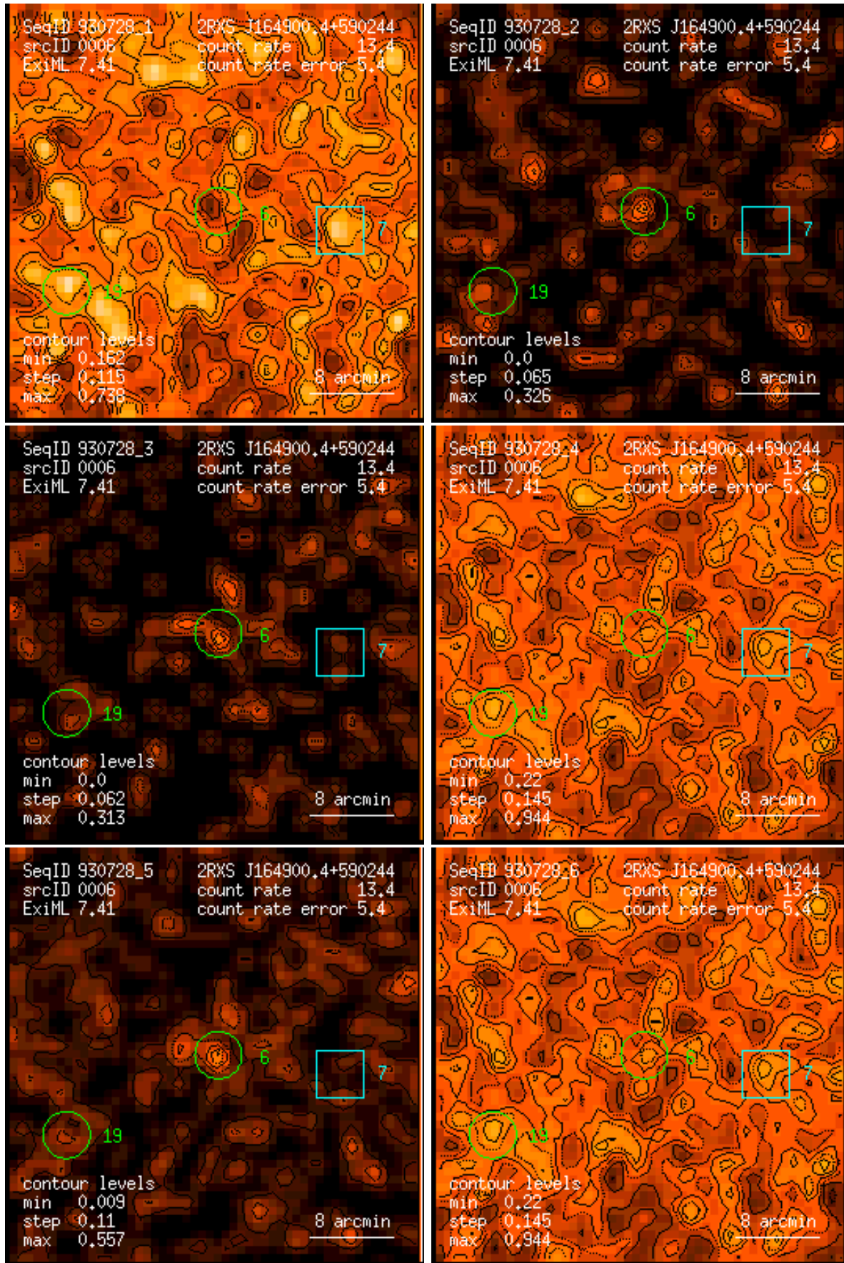
Figure 6: RASS 930728: detection 0006: band rate images, Gaussian filter: (1) PSPC channels 11 – 41, (2) 52 – 90, (3) 91 – 201, (4) 11 – 235, (5) 52 – 201, (6) 11 – 201. Broad band rates in counts/ks. Band rate contour levels in counts/ks/arcmin 2 .
