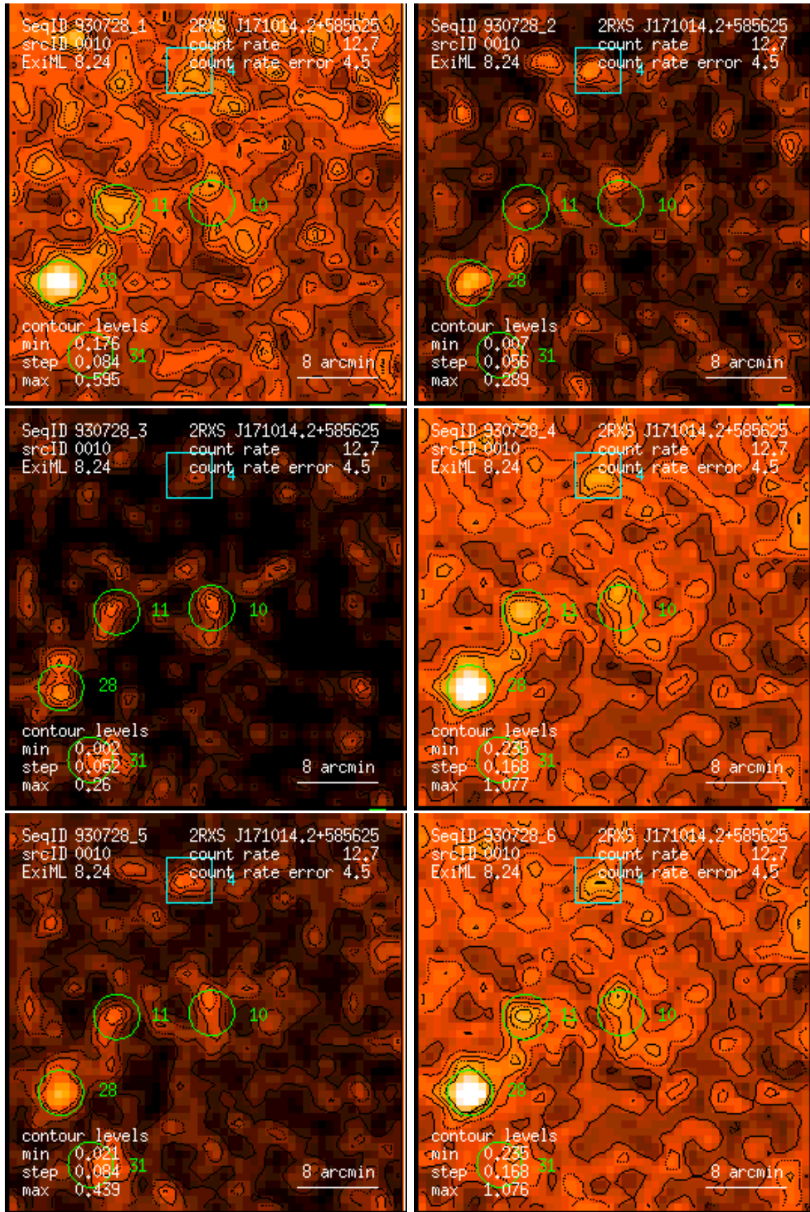
Figure 10: RASS 930728: detection 0010: band rate images, Gaussian filter: (1) PSPC channels 11 – 41, (2) 52 – 90, (3) 91 – 201, (4) 11 – 235, (5) 52 – 201, (6) 11 – 201. Broad band rates in counts/ks. Band rate contour levels in counts/ks/arcmin 2 .
